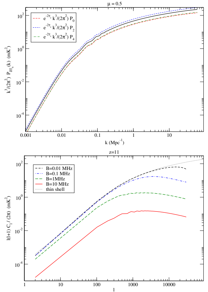
FIG. 3 (color online). Three-dimensional power spectra \mathcal{P}_{\delta T_b}(k) (top) and angular power spectrum C_\ell (bottom) for an observation redshift z = 11 and assuming no foregrounds. The cosmological parameters are the ones of Sec. II B ( \tau = 0.088 , z_{\text{reio}} \simeq 10.54 , x_{\text{H}} \simeq 0.87 , T_s \simeq 1360 K). The C_\ell are convolved with Gaussian window functions whose standard deviation is given by the bandwidth B . Large bandwidths damp the overall power but render the acoustic oscillations visible [42]. The thin shell limit has been obtained by integrating Eq. (24).
