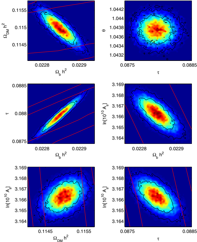
FIG. 14 (color online). Two-dimensional marginalized probability distribution for the combined four redshifts' FFTT and Planck-like CMB data. The inner black solid lines are the one- and two-sigma confidence intervals, the shading traces the mean likelihood. The outer red lines are the one- and two-sigma confidence intervals for four redshifts' FFTT data alone. The precise determination of \Omega_b h^2 from CMB strongly reduces the (\tau, \Omega_b h^2) correlations associated with the 21-cm signal.
