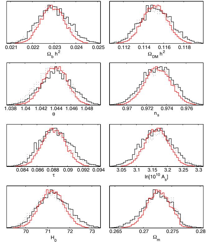
FIG. 10 (color online). Marginalized posteriors (solid) and mean likelihood (dotted) from two and four observation redshifts at reionization. The black outer curves are for two redshift slices z = 11, z = 12 while the red inner ones for four redshift z = 10, z = 11, z = 12 , and z = 13 (see also Fig. 11).
