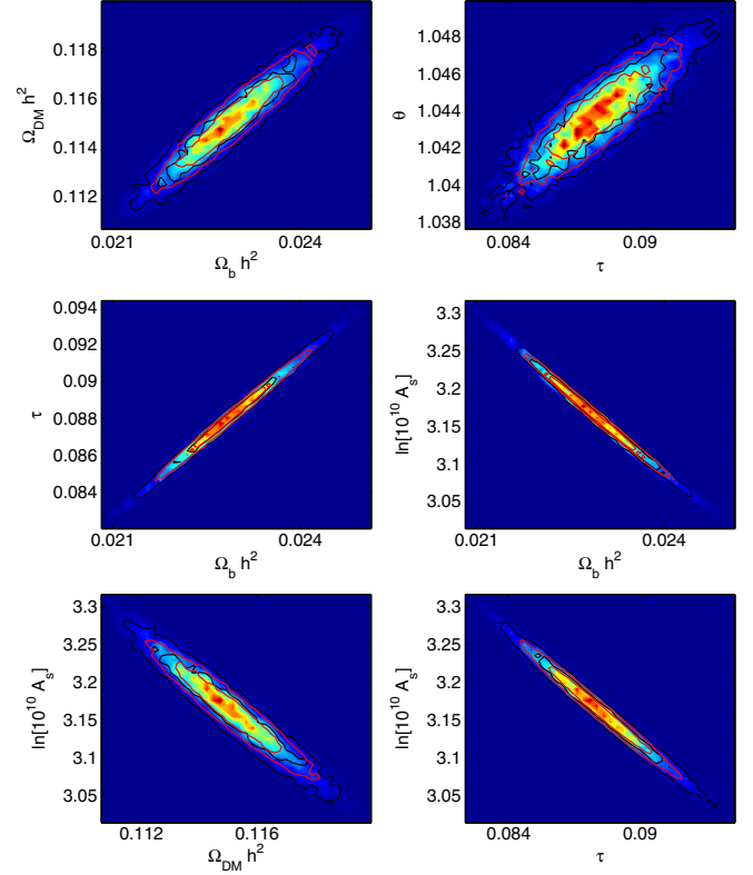
FIG. 11 (color online). Two-dimensional posteriors obtained by combining the FFTT data from multiple redshift slices. The shading traces the mean likelihood associated with the combination of two redshifts z = 11 and z = 12 . The black largest contours are the associated one- and two-sigma confidence intervals whereas the smaller red/gray contours are those associated with combined data for four redshifts ( z = 10, z = 11, z = 12 and z = 13 ). The degeneracies induced by \tau are accordingly reduced.
