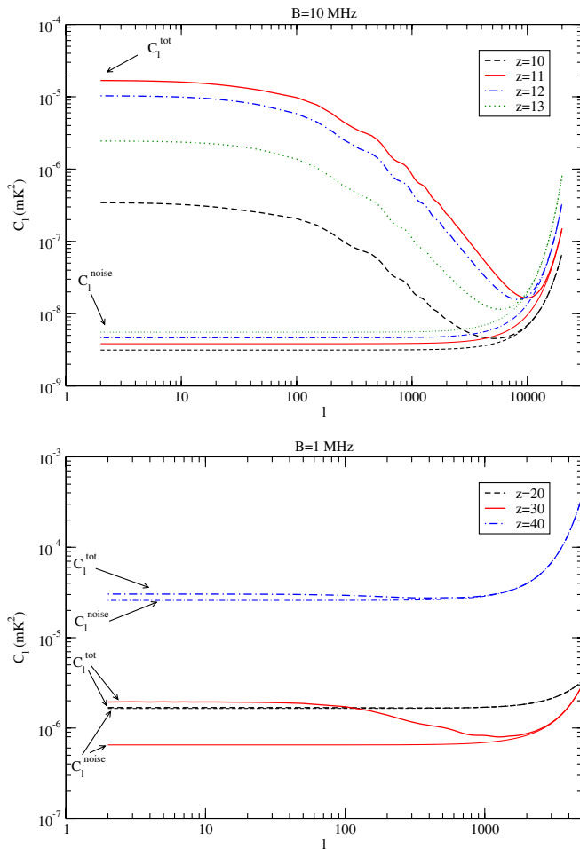
FIG. 5 (color online). Mock angular total power spectra C_\ell + C_\ell^{\text{noise}} and C_\ell^{\text{noise}} in \text{mK}^2 for various observation redshifts around reionization (top) and at the end of the dark ages (bottom). The cosmological parameters are the ones of Sec. II B ( \tau = 0.088 , z_{\text{reio}} \approx 10.5 ). The window functions are Gaussian in frequency space with a respective bandwidth of B = 10 MHz (top) and B = 1 MHz (bottom). The FFTT design is for D = 10 km and allows probing the dark ages for z \lesssim 30 , above which ionospheric absorption damps the signal (see z = 40 ).
