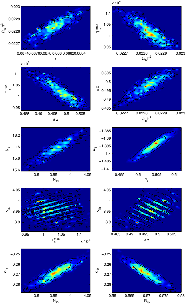
FIG. 18 (color online). Two-dimensional posterior probability distributions in the presence of the ionizing power spectra. The correlations induced by the nuisance parameter N_{ib} severely damages the expected constraints on the background reionization parameters \Delta_z and T_s^{\max} . The multivalued confidence intervals are the results of the acoustic oscillations (see text).
