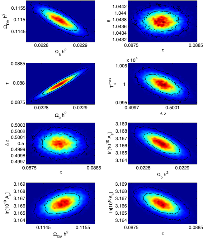
FIG. 16 (color online). Two-dimensional posterior probability distributions associated with the combined FFTT four redshifts' and Planck-like CMB data (see also Fig. 15). The background reionization model parameters, \tau , \Delta z and T_s^{\max} are weakly correlated and well reconstructed.
