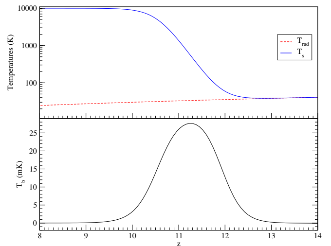
FIG. 2 (color online). Reionization driven spin temperature (top) and brightness temperature (bottom) with respect to the observation redshift. The reionization model is described in Sec. II B ( \tau = 0.088 ).
