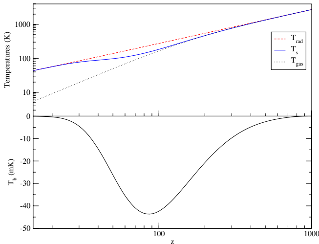
FIG. 1 (color online). Background evolution of the neutral hydrogen gas and spin temperatures (top) as a function of the redshift during the dark ages. The spin temperature T_s being defined as n_1/n_0 = 3 \exp[-\hbar\omega_{21}/(k_B T_s)] where n_0 and n_1 denote the number density of atoms in the singlet and triplet hyperfine states, respectively. The bottom panel shows the resulting brightness temperature.
