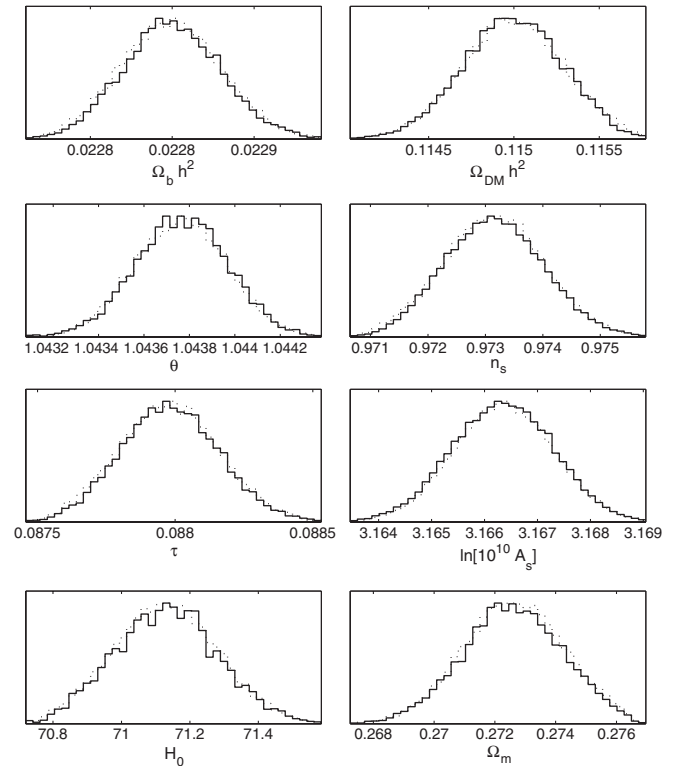
FIG. 13. Marginalized posteriors from the combination of the FFTT four redshifts' data ( z = 10 , z = 11 , z = 12 and z = 13 ) with Planck-like CMB data. The reduced variance on \Omega_b h^2 coming from CMB data kills most of the degeneracies associated with the 21-cm signal. Four redshifts' FFTT without CMB is represented in Fig. 10.
