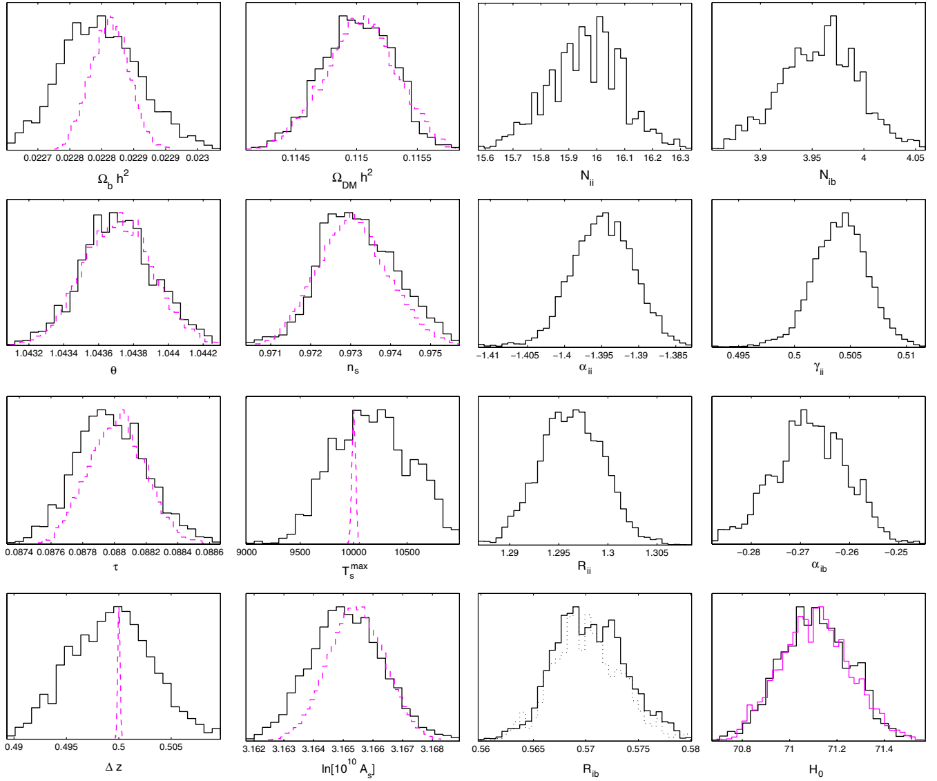
FIG. 17 (color online). Posterior probability distributions in the presence of the ionizing power spectra. The background reionization model has three varying parameters, \tau , \Delta_z and T_s^{\max} while the ionizing spectra involves seven nuisance parameters N_{ii} , \alpha_{ii} , \gamma_{ii} , R_{ii} , N_{ib} , \alpha_{ib} and R_{ib} . The posteriors of Fig. 15 have been reported as dashed curves to ease comparison.
