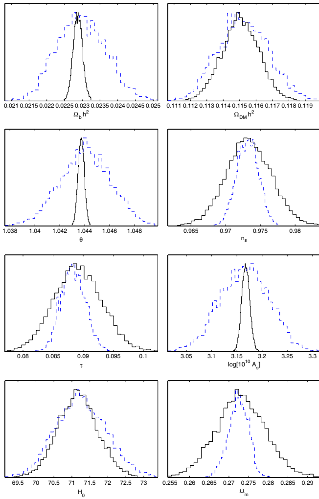
FIG. 12 (color online). Typical marginalized posterior distributions for a Planck-like CMB experiment (black solid lines). The dashed blue curves are the two redshift forecasts for FFTT (same as in Fig. 10).
