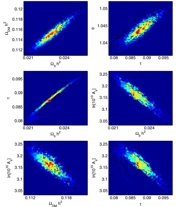
FIG. 9 (color online). Two-dimensional posteriors for a single observation redshift at z = 11 . The solid lines represent the one- and two-sigma confidence interval while the shading traces the two-dimensional mean likelihood. Notice the strong degeneracies induced by \tau which boost the expected variance on \Omega_b h^2 , for instance.
