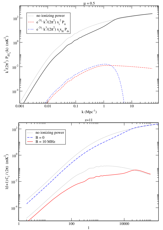
FIG. 4 (color online). Effects of the reionization power spectra at z = 11 (see Table I) on the three-dimensional power spectrum \mathcal{P}_{\delta T_b} (top). The bottom panel shows the reionization induced deviations on the angular power spectrum C_\ell , both for the thin shell approximation and a window function of bandwidth B = 10 MHz.
