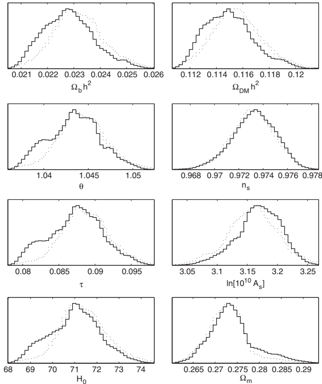
FIG. 8. Expected marginalized posterior probability distributions (solid) and mean likelihood (dotted) from a single redshift observation at z = 11 (reionization). The non-Gaussian posteriors and “shoulders” apparent for some parameters come from the large correlations induced by \tau (see Fig. 9).
