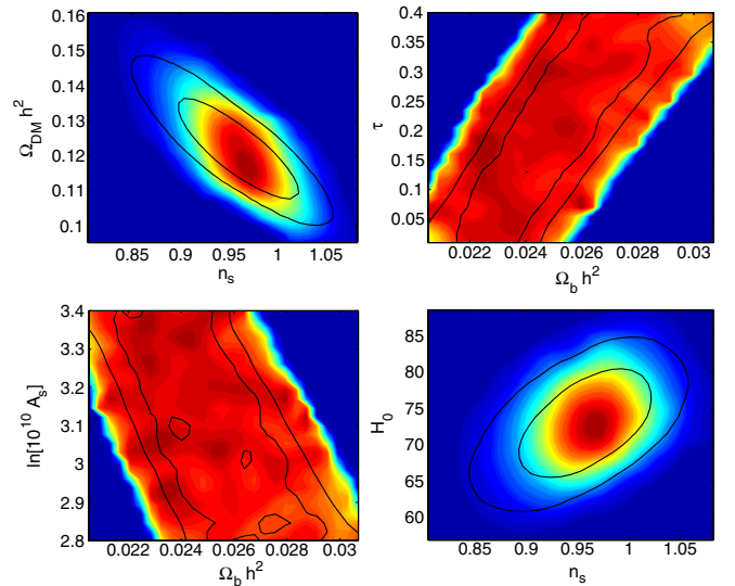
FIG. 7 (color online). One- and two-sigma confidence interval of the two-dimensional marginalized posterior probability distributions (solid lines) for a 10-km FFTT design at z = 30 . The shading traces the two-dimensional mean likelihood.
