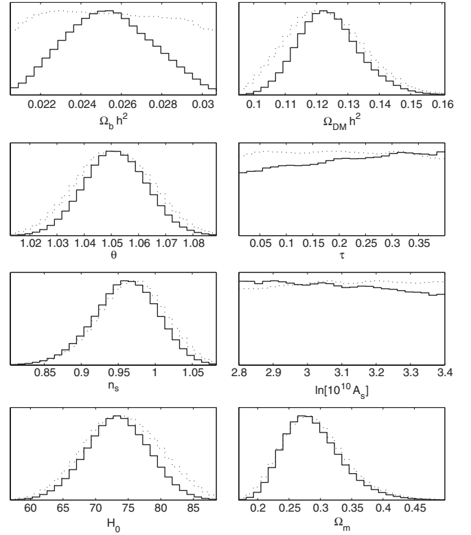
FIG. 6. Expected marginalized posterior probability distributions (solid) and mean likelihood (dotted) for 10-km FFTT data alone, at z = 30 (dark ages). The total optical depth \tau , primordial amplitude A_S , baryon density \Omega_b h^2 are completely degenerated and not constrained (see text and Fig. 7).
