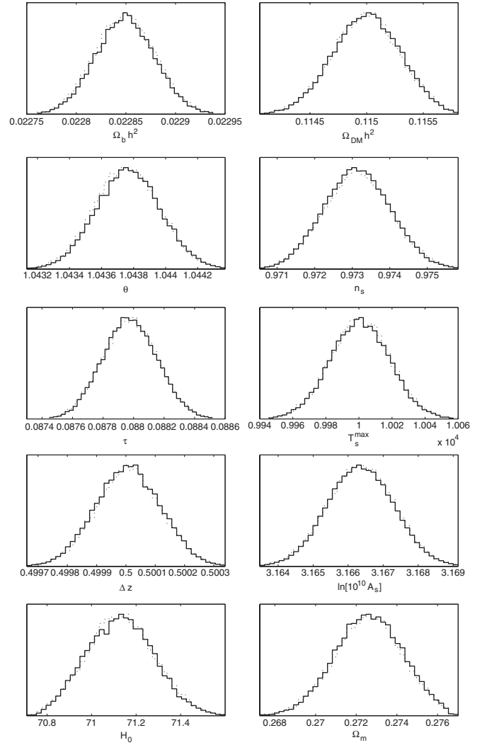
FIG. 15. Posterior probability distributions from combined FFTT four redshifts' and Planck-like CMB data. The background reionization model has three varying parameters, \tau , \Delta z and T_s^{\max} , all well reconstructed.
