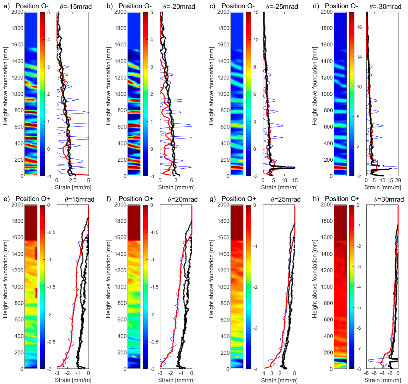
Figure 12. DIC and DFOS longitudinal strain profiles for the west web-flange intersection of wall unit UW2 subjected to torsion, in tension (Position O−): (a) \theta = -15 mrad; (b) \theta = -20 mrad; (c) \theta = -25 mrad; (d) \theta = -30 mrad, and in compression (Position O+); (e) \theta = 15 mrad; (f) \theta = 20 mrad; (g) \theta = 25 mrad; and (h) \theta = 30 mrad. The thin blue lines are the uncorrected strains determined from the DIC data, whereas the thick red lines are the corrected strains (i.e., moving average over 200 mm) determined from the DIC data. The solid black lines are the strain measurements from the DFOS (i.e., 2 \times \Phi 12 rebars, Channel 1). A heatmap is provided next to each plot, representing the uncorrected, raw DIC strain (in units of mm/m).
