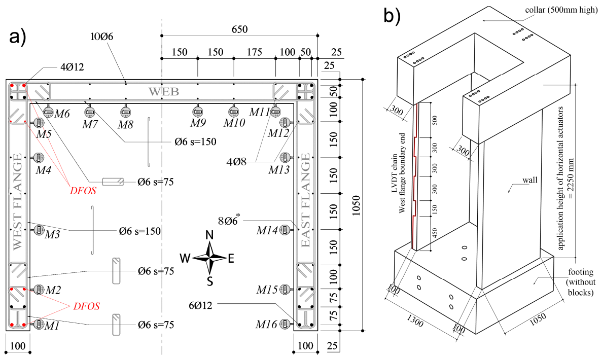
Figure 1. (a) Cross-section and reinforcement layout with indication of DFOS rebars and micrometer instruments (M1–M16, clockwise from boundary end of west flange); and (b) Elevation view of wall units with indication of the LVDT chain on the west flange boundary end.
