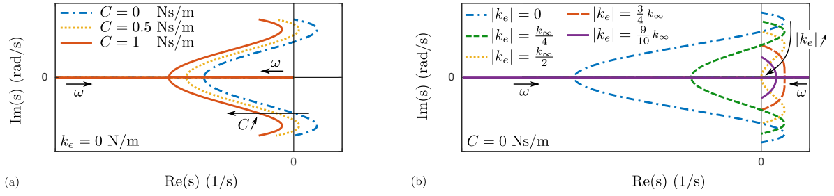
Figure 3. Root locus of both relevant eigenvalues. (a) Evolution with the damping C = \{0, 0.5, 1\} Ns/m for k_e = 0 N/m. (b) Evolution with the external stiffness |k_e| = \{0, \frac{1}{4}, \frac{1}{2}, \frac{3}{4}, \frac{9}{10}\} k_\infty N/m for C = 0 Ns/m.
