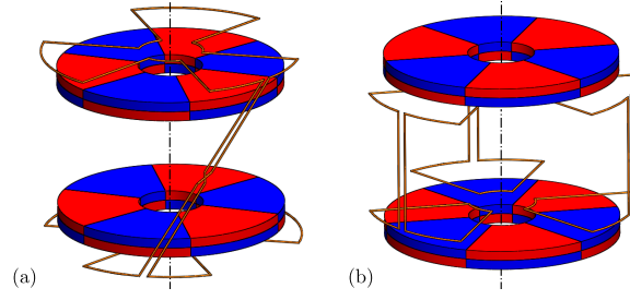
Figure 1. Bearing topologies with only one phase represented. (a) PMs are internal and the p coils of each set are connected in series, the two resulting sets being connected together in series. (b) PMs are external and the p upper and the p lower coils are independently connected together in opposition.
