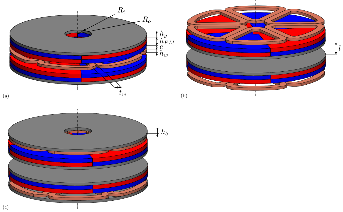
Figure 9. Study case: bearing topologies. (a) Topology 1. (b) Topology 2. (c) Topology 3.
