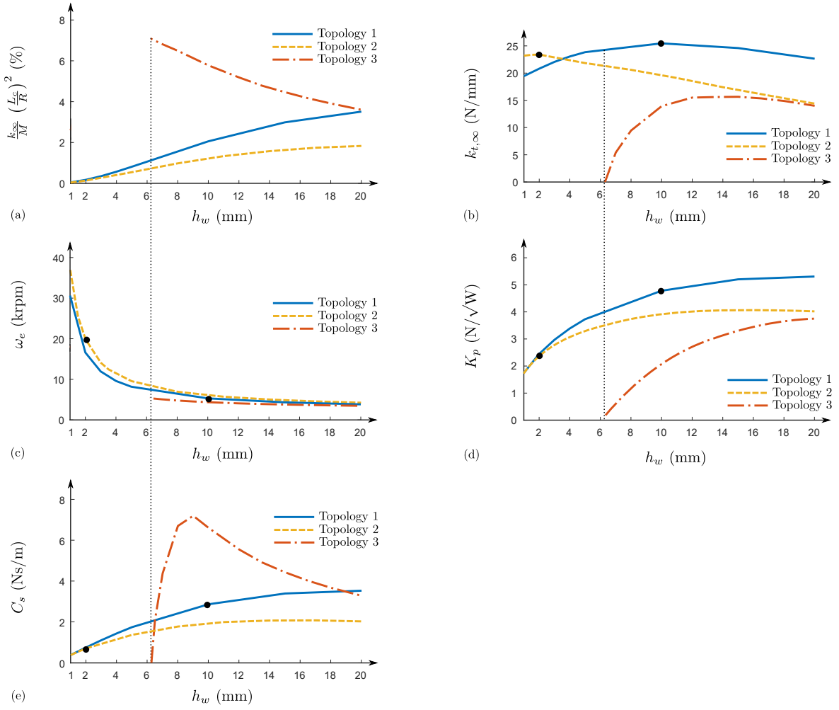
Figure 10. Study case: evolution of the performance criteria with the winding thickness for the three topologies. (a) Hypothesis validation. (b) Maximal total stiffness. (c) Spin speed related to the electrical pole. (d) Energy efficiency coefficient. (e) Stability margin.
