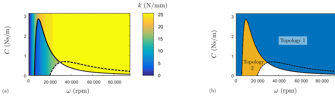
Figure 11. Study case: comparison of the stiffness of topologies 1 and 2 while taking into account their stability boundaries (solid and dashed lines respectively). (a) Maximal stiffness with the spin speed. (b) Corresponding topology.
