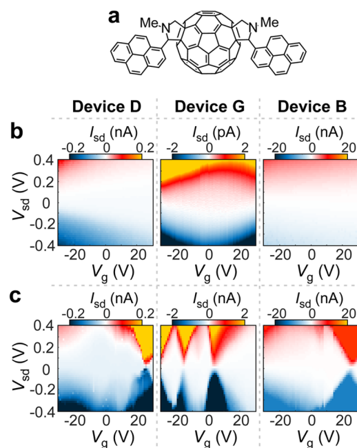
Figure 2. Electrical characterization of graphene–fullerene single-molecule thermoelectric nanodevices. (a) Chemical structure of the C 60 bisadducts functionalized with pyrene anchor groups. (b) Current map as a function of back gate and bias voltage before and (c) after molecule deposition recorded at T_0 = 77 K for devices D, G, and B, respectively.
