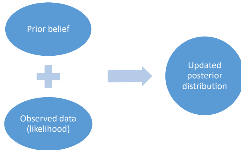
Figure 2-5: Bayesian framework
