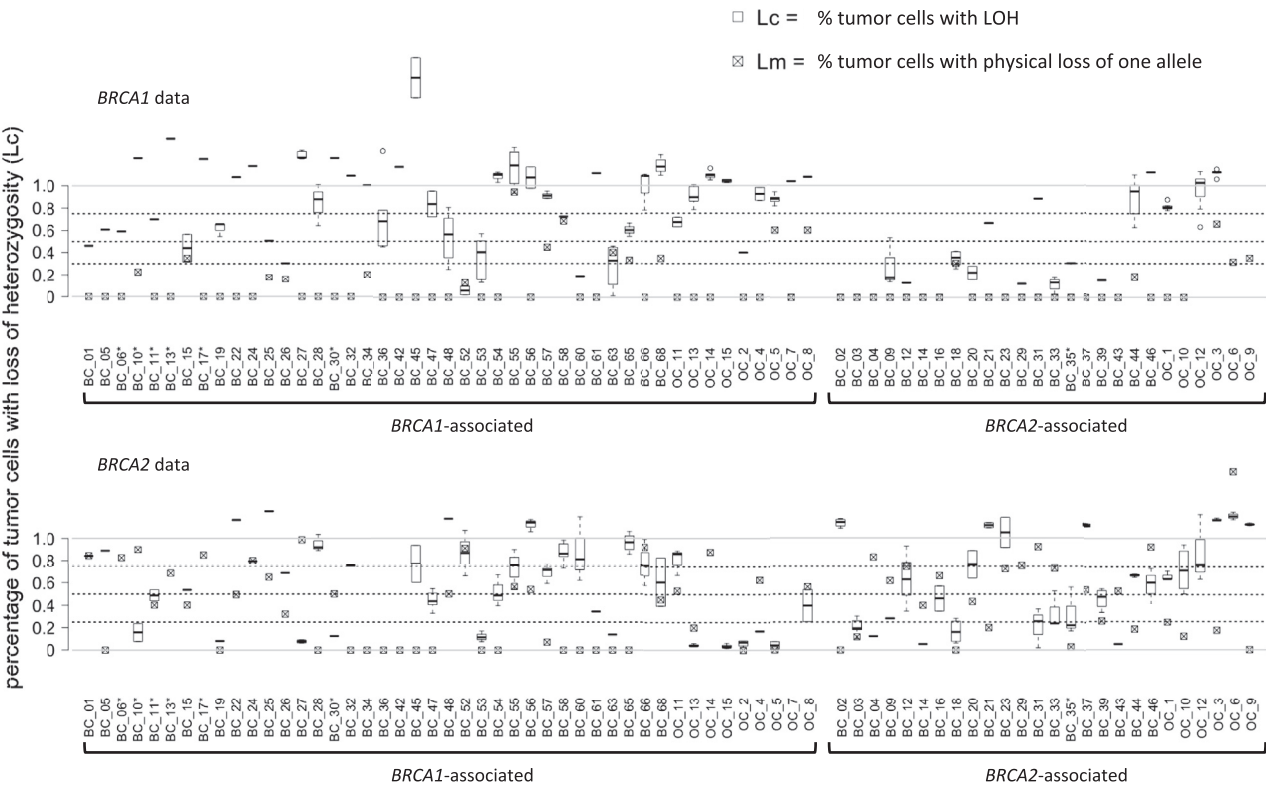
Fig. 3. Integrated LOH analysis using both sequencing and MLPA data. Boxplots represent Lc values (percentage of tumor cells in a sample that show LOH) for all germline heterozygous markers found in each sample as determined by sequencing. No correction was done on Lc values, as it is impossible to tell which factor (tVAF, bVAF or TCP) was responsible for the over- or underestimation of Lc. BRCA1 and BRCA2 are depicted in the upper and lower plots respectively. Samples with an asterisk indicated loss of the mutant allele. Lm values (percentage of tumor cells displaying physical loss of an allele as determined by MLPA) are represented as checked square boxes.
