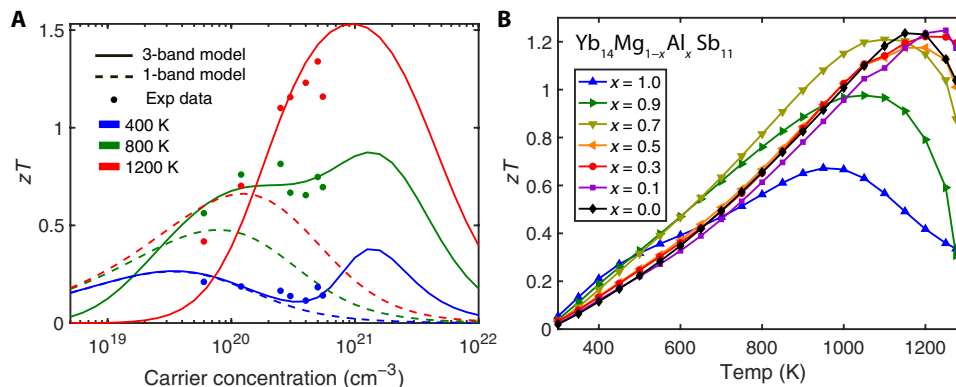
Fig. 7. Carrier concentration dependence of zT . (A) zT versus carrier concentration for \text{Yb}_{14}\text{Mg}_{1-x}\text{Al}_x\text{Sb}_{11} ( x = 0.0, 0.1, 0.3, 0.5, 0.7, 0.9, 1.0 ) compared with a single parabolic band model and the three-band model described here. While a single parabolic band model can describe low-temperature data reasonably well, it completely fails at predicting the temperature-dependent data and at instructing experimentalists the ideal carrier concentration to dope their materials. The work done here suggests that increasing the carrier concentration of \text{Yb}_{14}\text{MgSb}_{11} could lead to even further enhancement in the material's zT . (B) Temperature-dependent zT . The samples with the highest carrier concentration ( x = 0.1 and 0.3 ) have the highest zT .
