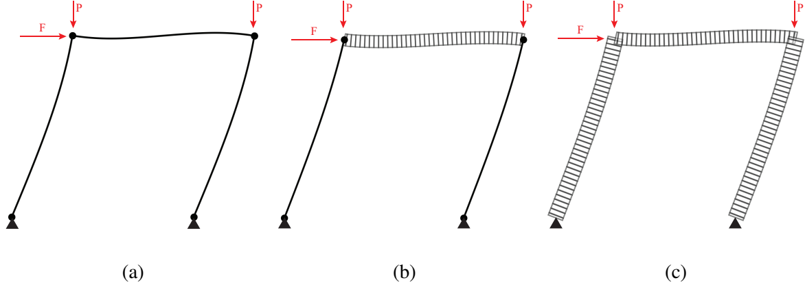
Figure 4: (a) full FEM model (b) coupled HybridFEM (beam)- FEM (columns) model (c) full HybriDFEM model at a horizontal displacement of 5 cm. The deformations are magnified by a factor of 20.
