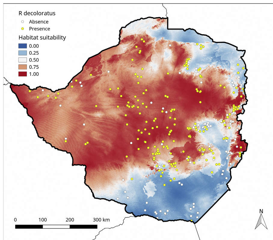
Fig. 2. Habitat suitability map for Rhipicephalus decoloratus in Zimbabwe.
