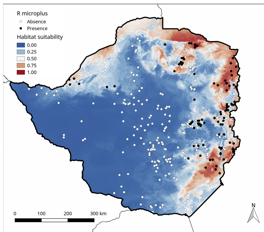
Fig. 1. Habitat suitability map for Rhipicephalus microplus in Zimbabwe.
