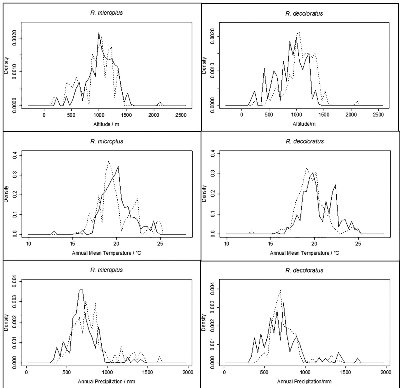
Fig. 4. Probability density distributions of altitude, annual mean temperature and annual precipitation with respect to the presence (dashed line) and absence (continuous line) of Rhipicephalus microplus and R. decoloratus in Zimbabwe.
