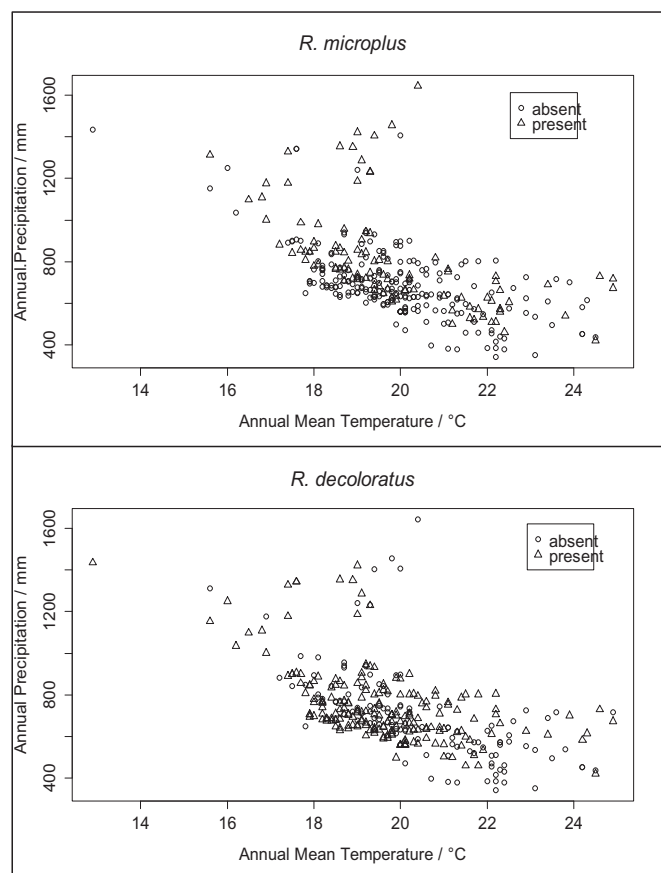
Fig. 5. Bi-plot showing annual mean temperature and annual precipitation with respect to presence or absence of Rhipicephalus microplus and R. decoloratus in Zimbabwe.
