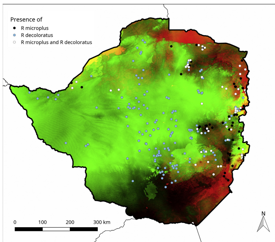
Fig. 2. Habitat suitability map for Rhipicephalus decoloratus in Zimbabwe.
