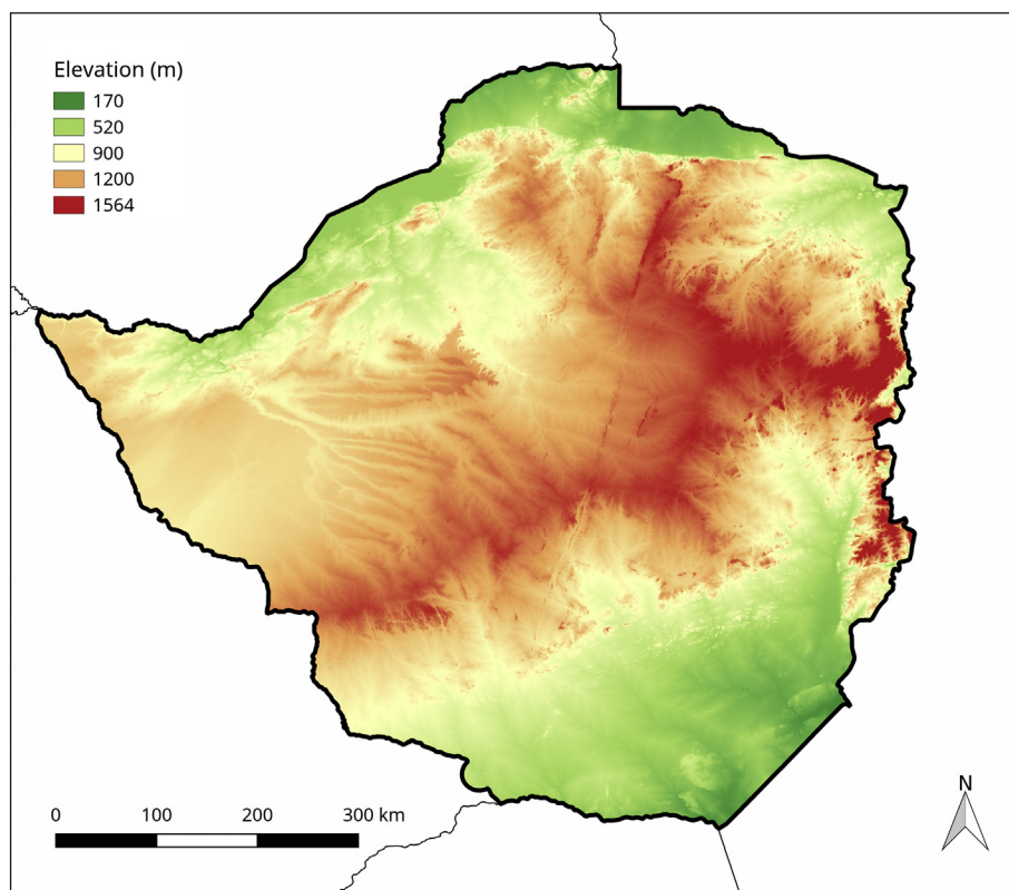
Fig. 6. : Map showing variation in altitude (m) in Zimbabwe based on WorldClim data.
