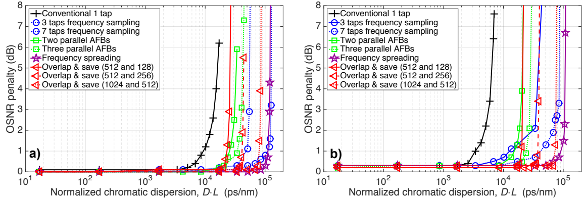
Fig. 5. OSNR penalty as a function of the normalized CD for a) 4-OQAM and b) 16-OQAM modulations.
