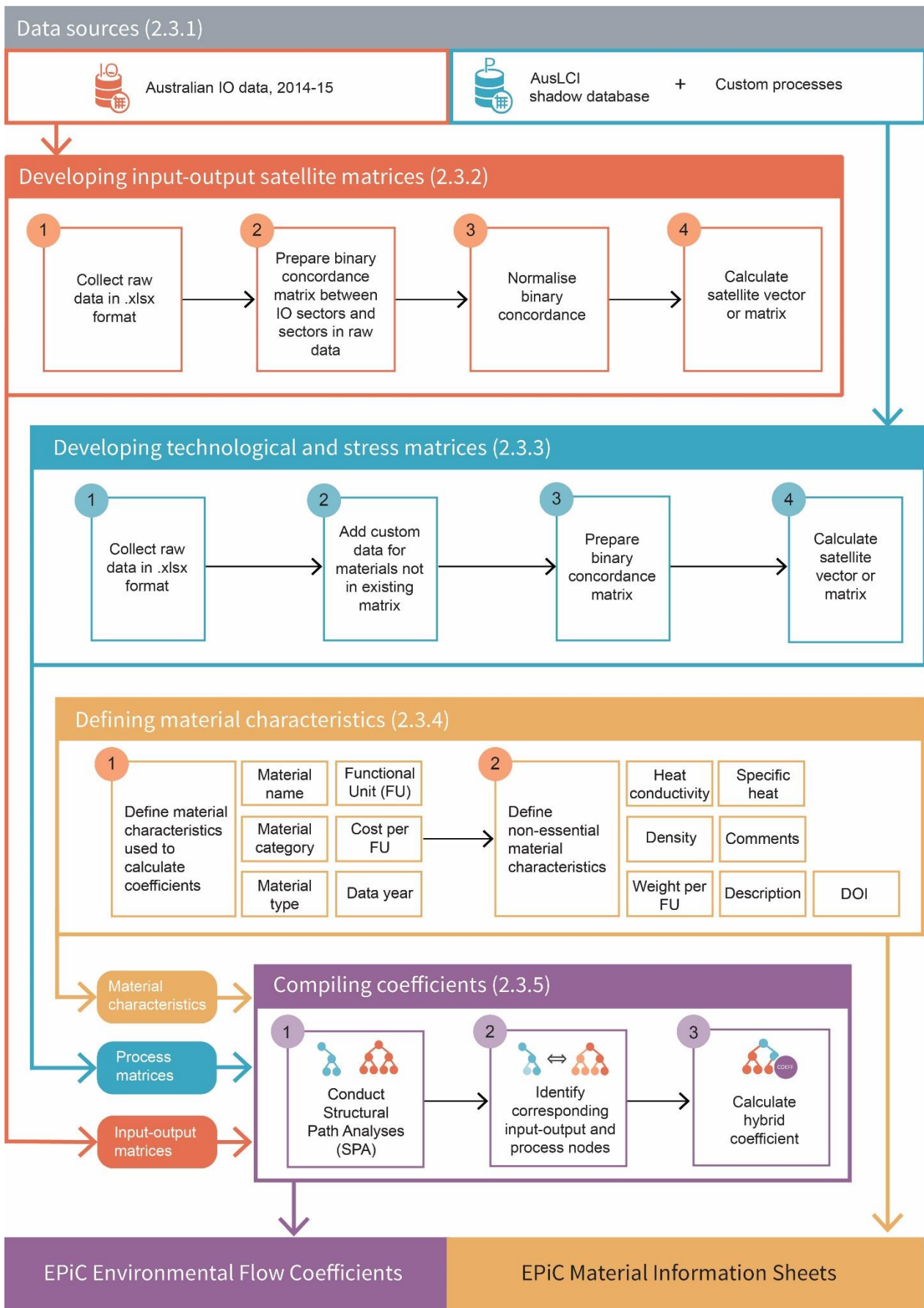
Figure 1: Steps in creating the EPiC Database
