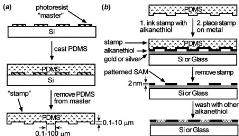
Figure 1.20 – Stamp fabrication in soft lithography and microcontact printing application. (a) A photoresist master is patterned by photolithography, and PDMS is casted around the pattern on the substrate. After curing, the PDMS is removed and can act as a mold for printing. (b) A PDMS stamp is dipped into a solution containing alkanethiol and placed in contact with gold or silver on the substrate surface. The alkanethiol that has adsorbed to the stamp is allowed to react, resulting in a patterned self-assembled monolayer. The non-patterned areas can later be filled with a different alkanethiol [189].
