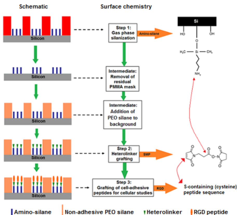
Figure III.2 – Surface functionalization schematic. After oxygen descum, the substrates are immediately subjected to a three-step surface functionalization process. In the exposed, nanopatterned regions, an amino-silane (APDMS) is grafted to the silicon substrate via reaction with the surface silanol groups. An acetone washing is then performed using a Soxhlet apparatus set-up for 2 hours to remove the remaining PMMA mask, as well as any excess amino-silane. A PEO silane is then grafted to the non-patterned regions of the substrates as a passivation step to render the background non-adhesive to cells and proteins. The second functionalization step is the grafting of a hetero-bifunctional cross-linker. In this case, 3-succinimidyl-3-maleimidopropionate (SMP) reacts with the amino-silane layer to form an amide bond. In the last step, a cell-adhesive RGD peptide, containing a cysteine in its sequence, is grafted to the SMP via thiol linkage with the maleimide group. This last operation is performed at a later stage, just before using the substrates for cell culture.
