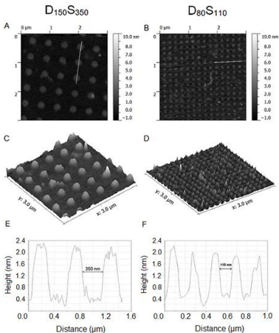
Figure IV.19 – AFM characterization of nanopatterned surfaces. Contact mode measurements performed on (A) D_{150}S_{350} and (B) D_{80}S_{110} surfaces. The nanosized features are grafted by SMP (hetero-bifunctional cross-linker). The difference in height between the background and the nanodots is indicative of topographical contrast between the SMP and the PEO layers. 3D reconstruction of the (C) D_{150}S_{350} and (D) D_{80}S_{110} surfaces was performed on an area of 3 \times 3 \mu\text{m}^2 to illustrate topography. Height profiles of the lines drawn in (A) and (B) are shown respectively in (E) and (F).
