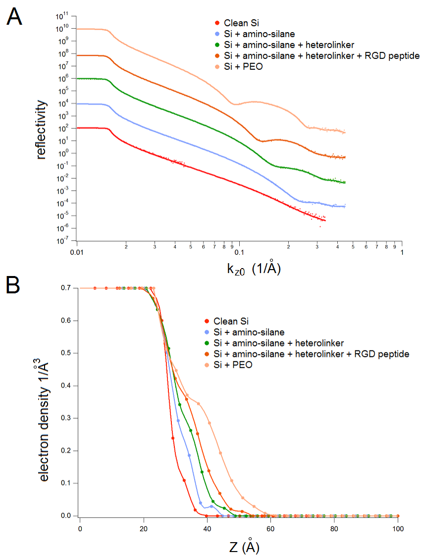
Figure IV.5 – XRR profiles during peptide grafting process. At each functionalization step, X-ray reflectivity (A) was measured and the electron density of the systems (B) was computed using procedures described elsewhere [234]. Evidently in (B), the thickness of the organic film increases with each grafting step, indicating that the successive deposition of molecules was achieved.
