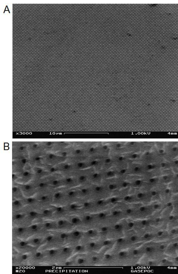
Figure IV.2 – Scanning electron microscopy characterization of (A) the master mold used for nanoimprint lithography to produce D_{150}S_{350} surfaces, imaged at 3000X magnification with scale bar = 10\mu\text{m} , and (B) nanoimprinted PMMA mask using the mold in (A), imaged at 20000X magnification with scale bar = 2\mu\text{m} .
