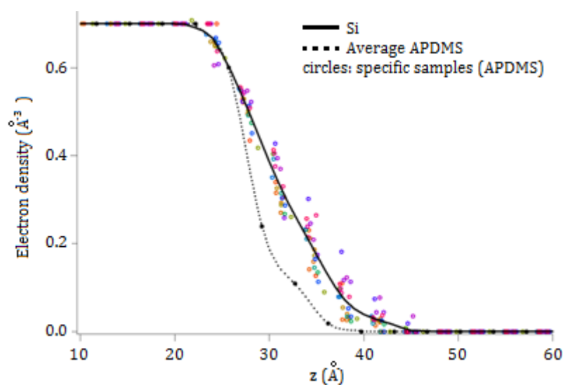
Figure IV.6 – XRR electron density profile of APDMS grafting. The circles represent data obtained from individual measurements after APDMS grafting, fitted with the black solid curve.
