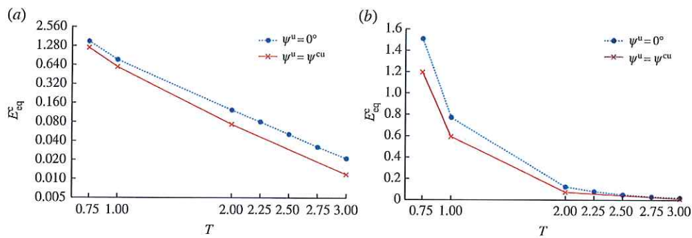
Figure 11. Variation the critical equivalent strain outside the band at first localization, E_{eq}^c , as a function of T for f_0 = 0.001 , L = -1 and N = 0.1 . The critical strain for the normal band orientation and for the critical band orientation are shown. The vertical axis uses a base 10 logarithmic scale for (a). (Online version in colour.)
