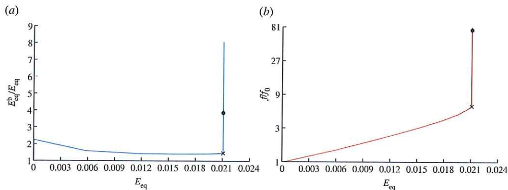
Figure 4. Evolution of (a) E_{eq}^b/E_{eq} , and (b) f/f_0 with E_{eq} for f_0 = 0.001 , T = 3.00 , L = -1 , N = 0.1 and \psi^u = 0^\circ . The vertical axis is plotted by using a base 10 logarithmic scale for (b). (Online version in colour.)
