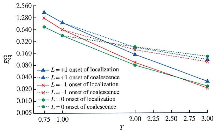
Figure 13. The dependence of the variation of the critical effective strains in the band, E_{eq}^{db} , with T on the Lode parameter, L , for f_0 = 0.001 , N = 0.1 , at the critical band orientation. The vertical axis is plotted by using a base 10 logarithmic scale. (Online version in colour.)
