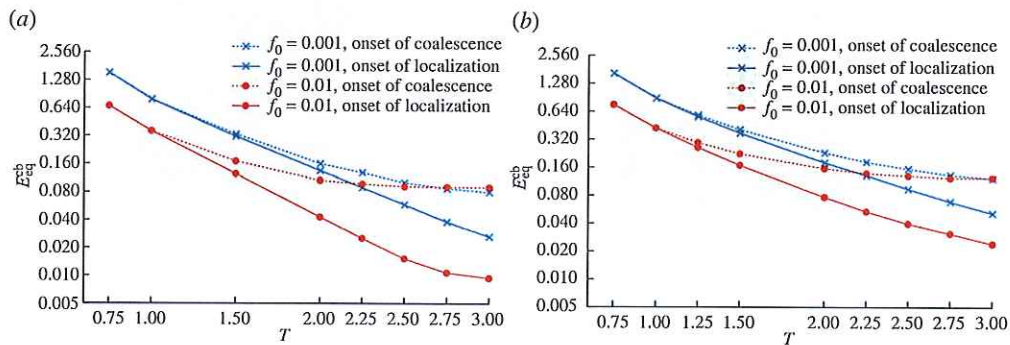
Figure 7. Values of E_{eq}^b at first localization and at the onset of coalescence as a function of T for L = -1 , \psi^u = 0^\circ ; N = 0.1 for (a), and N = 0.2 for (b). The vertical axis is plotted by using a base 10 logarithmic scale for both figures. (Online version in colour.)
