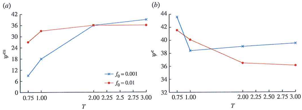
Figure 12. Variation with respect to T of the critical band orientation in the undeformed state, \psi^u , in (a) and in the deformed state, \psi^c , in (b) for L = -1 and N = 0.1 . (Online version in colour.)
