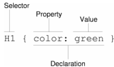
Figure 4.15: CSS rule structure
