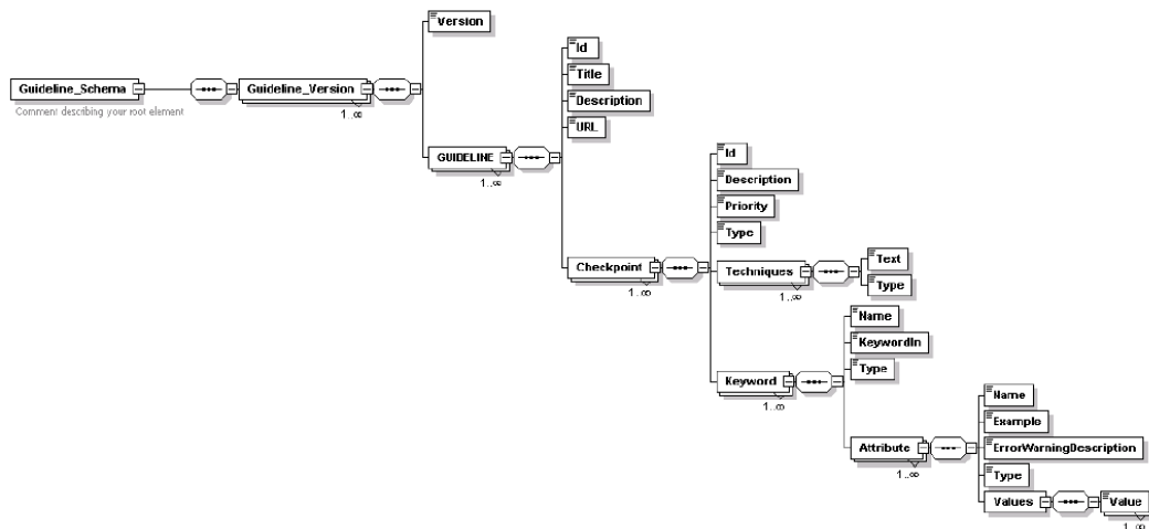
Figure 4.3: XML Schema for WAI guidelines as defined in Evallris
