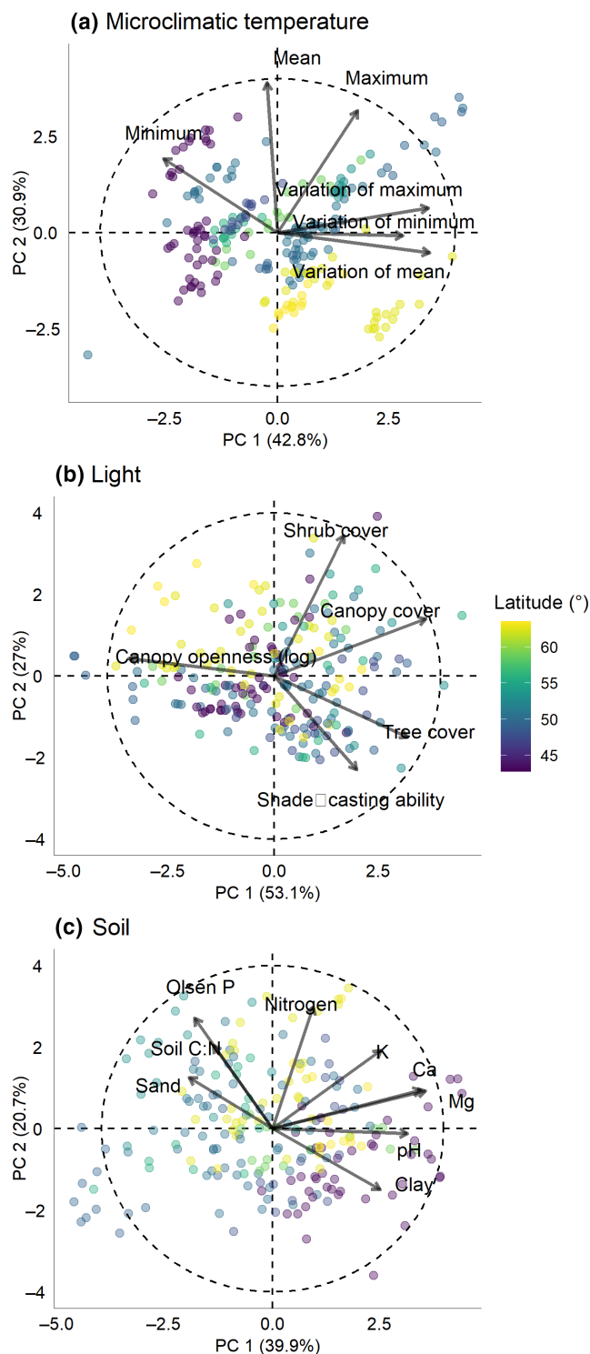
FIGURE 1 Principal components analysis plots for (a) air temperature, (b) light availability and (c) soil properties in temperate forest understoreys across Europe. The arrows indicate the relative loadings of each explanatory variable (scaled to a circle with radius 4 to improve visibility).
