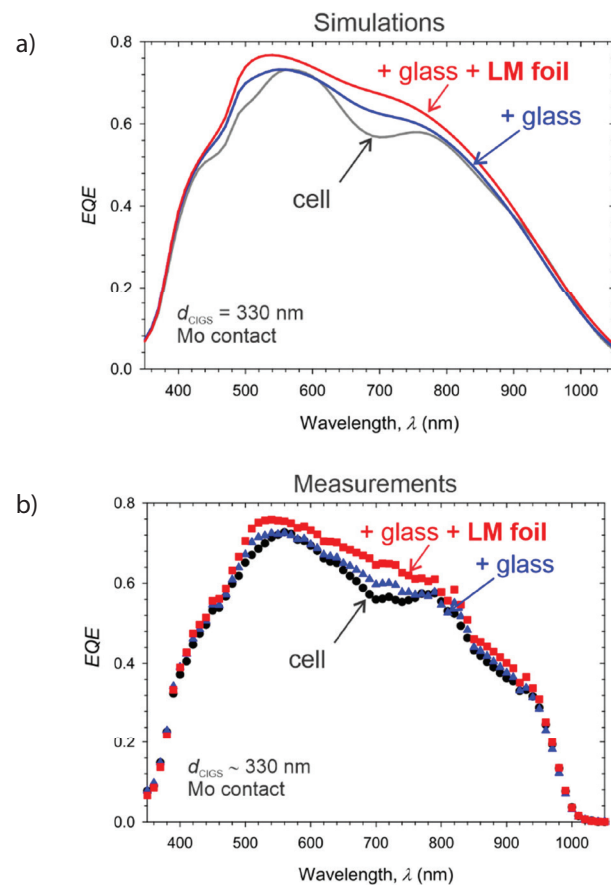
Figure 4: (a) Simulated and (b) measured EQE of an ultra-thin CIGS cell ( d_{CIGS} = 330 nm) in three configurations: bare cell (i) – black lines&symbols, with added front glass (ii) – blue lines&symbols and with added glass and LM foil (iii) – red lines&symbols. Differences in long wavelength range can be contributed to different bandgap of fabricated and simulated CIGS absorber.
