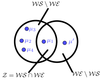
Fig. 1. Relation between WE , WS , and Z in Example 3.
