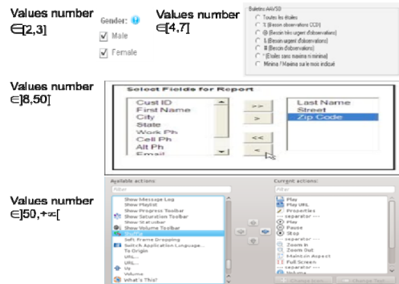
Fig. 6. A Multiple-choice widgets definition for a known domain [22]
