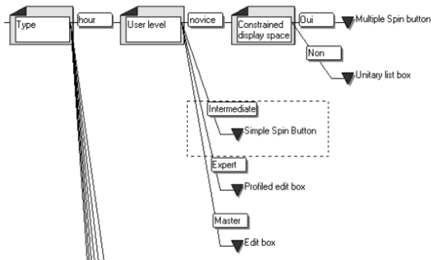
Fig. 5. A partial view of the TRIDENT's AIO Selection Tree [35]
