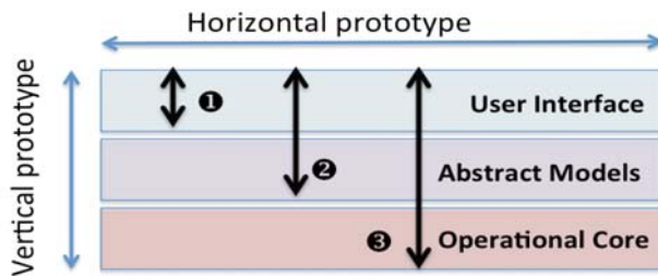
Fig. 10. Agile Adaptation in the support of OMP [34]
