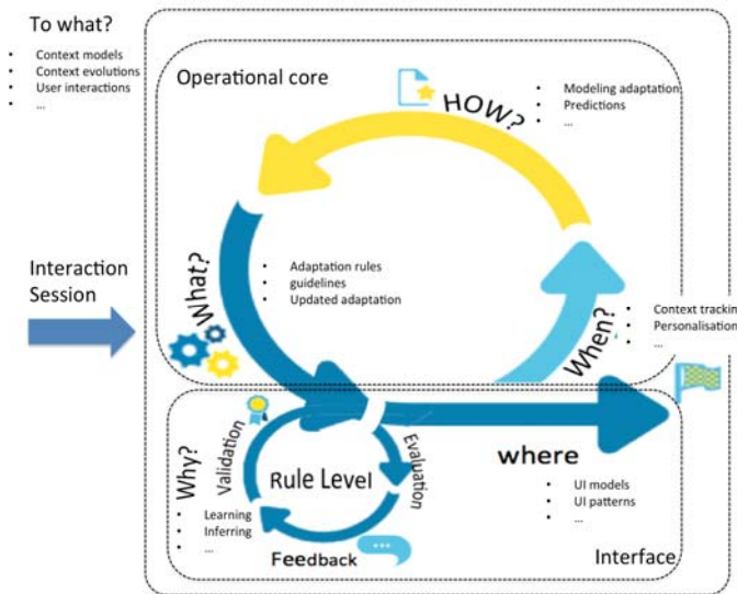
Fig. 9. Agile runtime adaptation lifecycle
