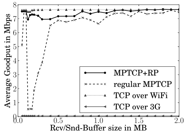
Figure 4.8: WiFi and a lossy 3G path - Retransmissions over 3G are very costly, but our mechanisms allow to overcome this limitation.
