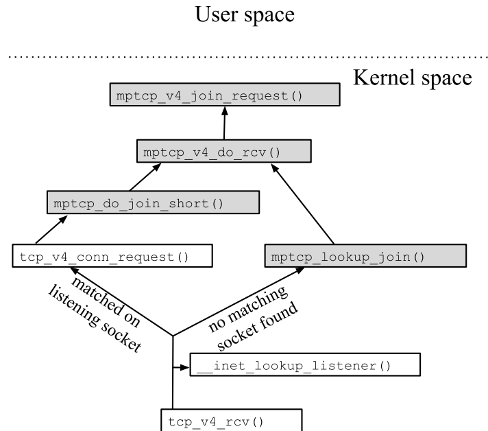
Figure 5.10: If the SYN + MP_JOIN matches on a listening socket, this code-path is being reused.
