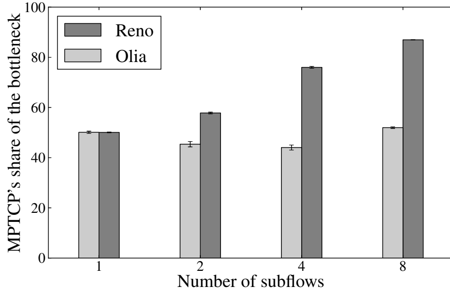
Figure 2.10: The Olia congestion control is fair to regular TCP across shared bottlenecks.
