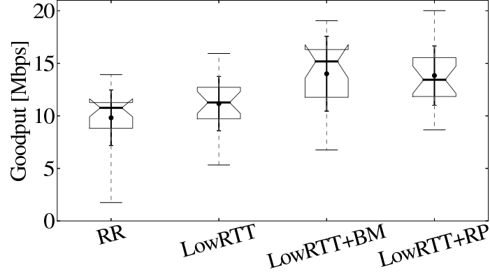
Figure 4.20: NorNet : With bounded buffers (2 MB), LowRTT+BM and LowRTT+RP achieve the best performance.
