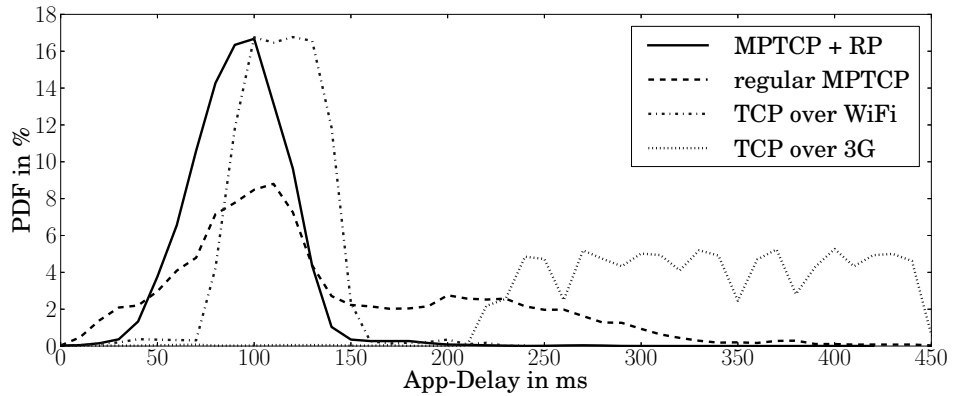
Figure 4.11: Application level latency for 3G/WiFi case
