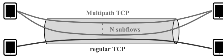
Figure 2.9: If regular TCP congestion control is being used, Multipath TCP would use much more capacity across shared bottlenecks and be unfair to regular TCP.
