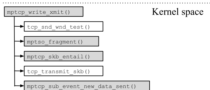
Figure 5.14: A simplified view of the different steps involved when transmitting data in Multipath TCP
