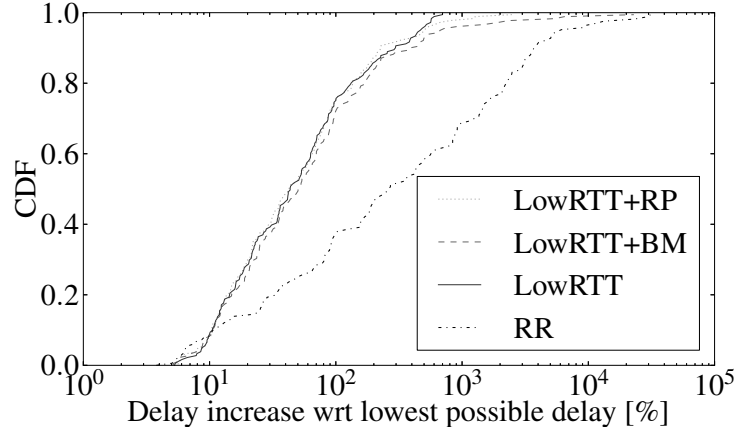
Figure 4.21: Mininet: Using the lowest-RTT-first scheduler greatly reduces the application-delay variance in Mininet.
