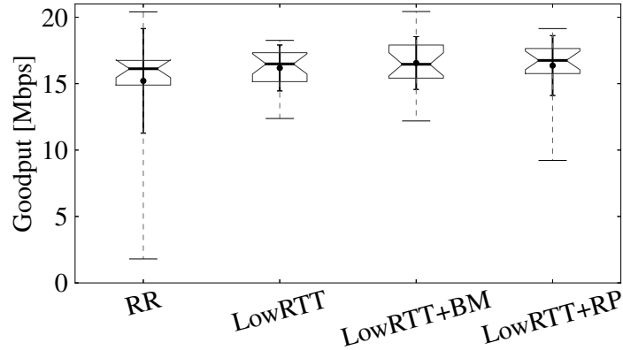
Figure 4.19: NorNet : With unbounded buffers (16 MB), each scheduler achieves the goodput.
