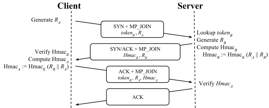
Figure 6.6: Handshake of a new subflow.
