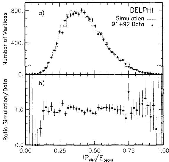
Fig. 11. a) \langle |P_{vis}| \rangle / E_{beam} for vertices used in this analysis and b) ratio of the simulation with respect to the data
