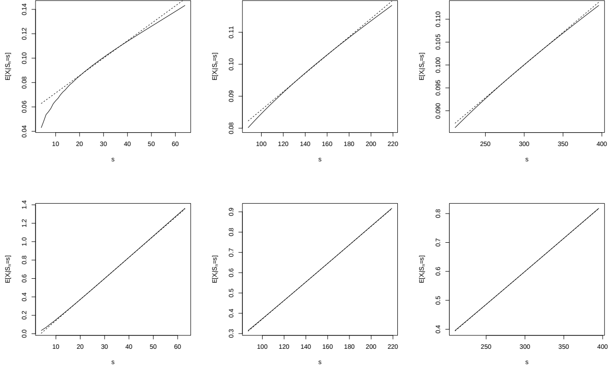
Figure 5: Functions s \mapsto E[X_i | S_n = s] (continuous line) and their large-pool approximation (broken line) for n = 100 (left panels), n = 500 (middle panels), and n = 1000 (right panels), and a participant in group 1 (upper panels) and in group 2 (lower panels) for the pool described in Example 4.3.
