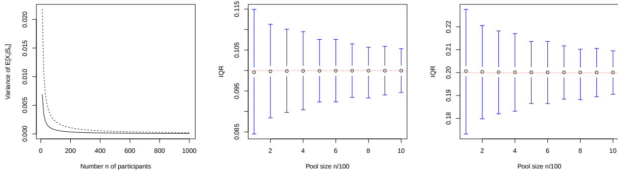
Figure 1: Variance of E[X_i|S_n] as a function of n \in \{10, 20, 30, \dots, 1000\} (left panel) for a participant in group 1 (continuous line) and in group 2 (broken line), median and interquartile range (IQR) of E[X_i|S_n] for n \in \{100, 200, 300, \dots, 1000\} in group 1 (middle panel) and in group 2 (right panel) for the pool described in Example 3.2. Horizontal lines in the central and right panels correspond to expected mortality credits.
