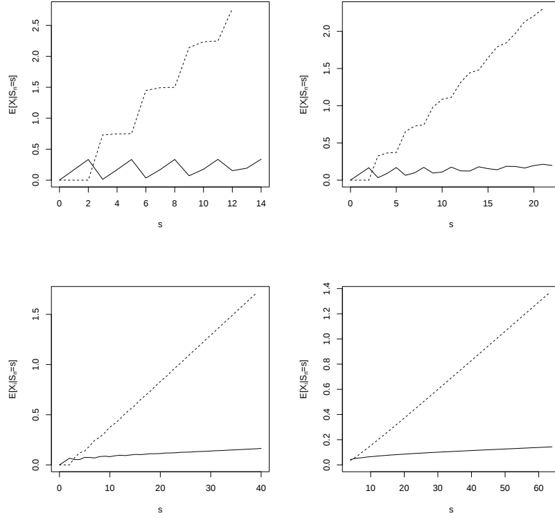
Figure 4: Functions s \mapsto E[X_i | S_n = s] for n = 10 (upper left panel), n = 20 (upper right panel), n = 50 (lower left panel), and n = 100 (lower right panel), for a participant in group 1 (continuous line) and in group 2 (broken line) in the pool described in Example 4.3.
