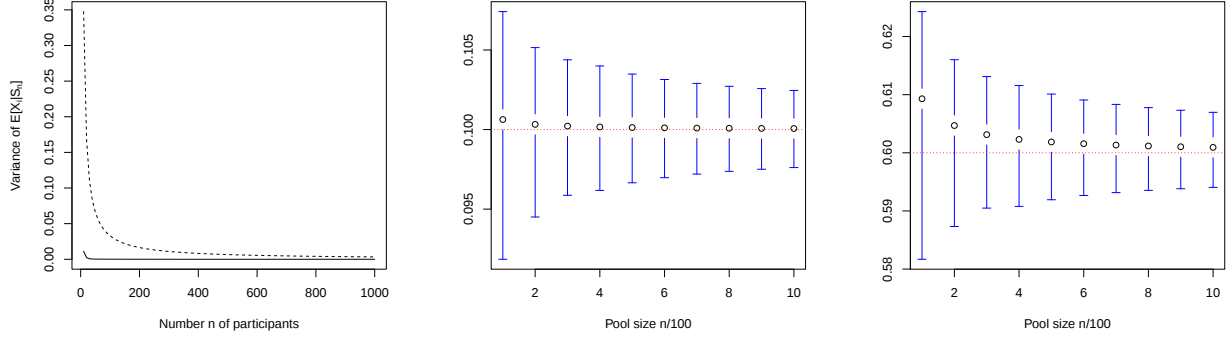
Figure 3: Variance of E[X_i|S_n] as a function of n \in \{10, 20, 30, \dots, 1000\} (left panel) for a participant in group 1 (continuous line) and in group 2 (broken line), median and interquartile range (IQR) of E[X_i|S_n] for n \in \{100, 200, 300, \dots, 1000\} in group 1 (middle panel) and in group 2 (right panel) for the pool described in Example 4.3. Horizontal lines in the central and right panels correspond to expected mortality credits.
