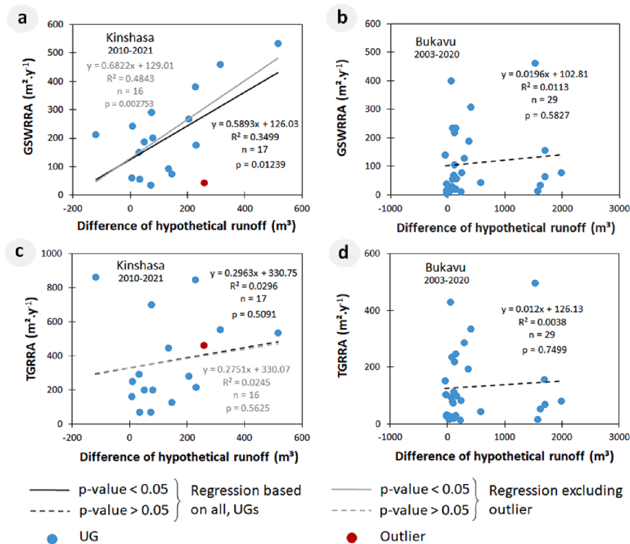
Fig. 9. Relationships between the difference in hypothetical runoff volume at the gully head (Eq. (9)) and average expansion rate of the urban gully (UG) over the entire measuring period. GSWRRA: areal gully sidewall widening retreat rate; TGRRA: areal total gully retreat rate. One point in Kinshasa (indicated in red) was considered to be an outlier (see section 3.2.1 for further details). (For interpretation of the references to colour in this figure legend, the reader is referred to the web version of this article.)
