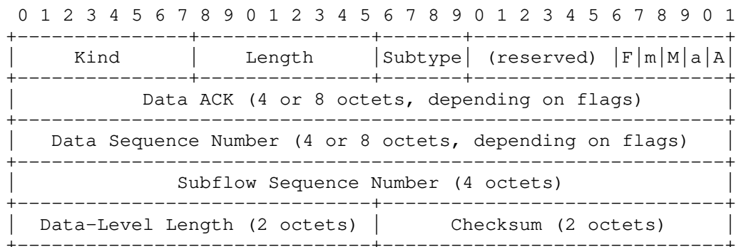
Figure 2: The DSS option in RFC8684
