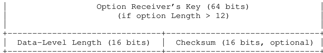
Figure 4: The MP_CAPABLE option
