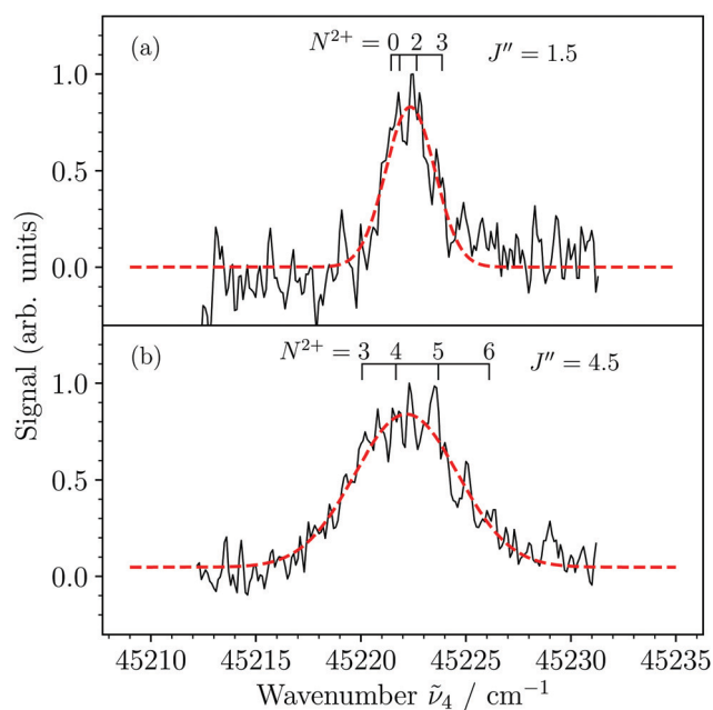
Fig. 6 MATI spectra of the X^{2+}(v^{2+} = 3, N^{2+}) \leftarrow 3d\pi_{1/2}^+(v'' = 3, J'') photo-ionizing transition generated by the third pulse of the pulse sequence +0.26, -1.12, -1.72 , and +172.4 \text{ V cm}^{-1} recorded with predominant population of the J'' = 1.5 (a) and 4.5 (b) rotational levels in the intermediate 3d\pi_{1/2}^+(v'' = 3) state. The assignment bars indicate transitions to the rotational levels of MgAr^{2+} assuming dominant branches with N^{2+} - J'' = -1.5, \dots, +1.5 .
