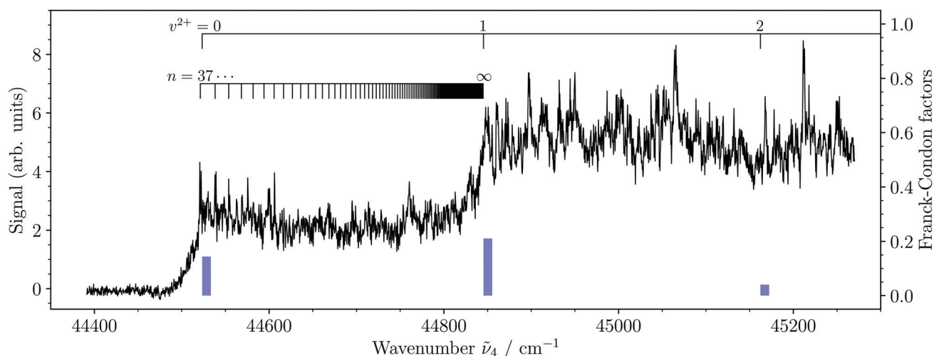
Fig. 4 Photoionization spectrum of \text{MgAr}^+ recorded from the intermediate 3d\pi_{1/2}^+(v''=2) level. The two intensity steps correspond to the first two ionization thresholds as indicated along the upper assignment bar. The lower assignment bar indicates the position of Rydberg states converging to the \text{MgAr}^{2+} X^{2+}(v^{2+}=1) threshold, several of which are observed as autoionizing resonances just above the X^{2+}(v^{2+}=0) level. The blue vertical bars represent the Franck-Condon factors (right vertical axis) calculated with the potential-energy functions of the 3d\pi_{1/2}^+ and X^{2+} states. See the text for details.
