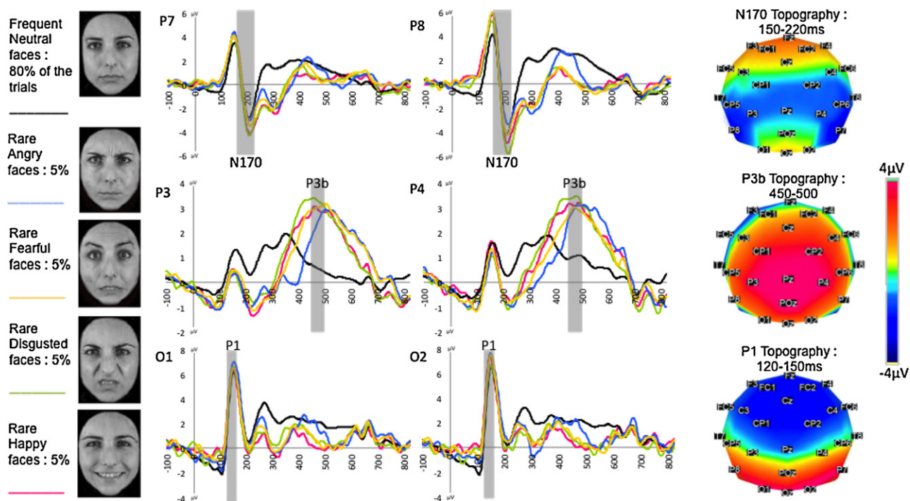
Fig. 1. Illustration of the five categories of stimuli, grand mean baseline corrected ERP time courses at P7, P8, P3, P4, O1 and O2 for the different types of stimuli (colour legend appears on the left of stimuli and time windows are indicated by grey boxes), and mean ERP topographies during rare stimuli processing.
