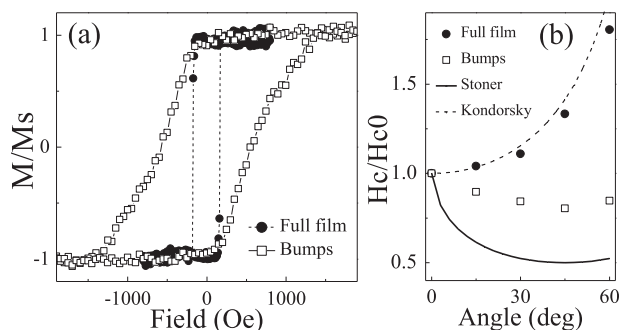
FIG. 3. (a) Hysteresis loops at 300 K, for Co/Pt multilayers with the field applied perpendicular to the bumpy (open squares) and flat (solid circles) substrates; (b) relative coercivity as a function of the angle of the field with respect to the anisotropy axis for the bumpy (open squares) and full film (solid circles) samples. H_{c0} corresponds to the coercive field measured with field parallel to the easy axis. The dashed and solid lines in (b) correspond to Kondorsky and Stoner–Wohlfarth models, respectively.
