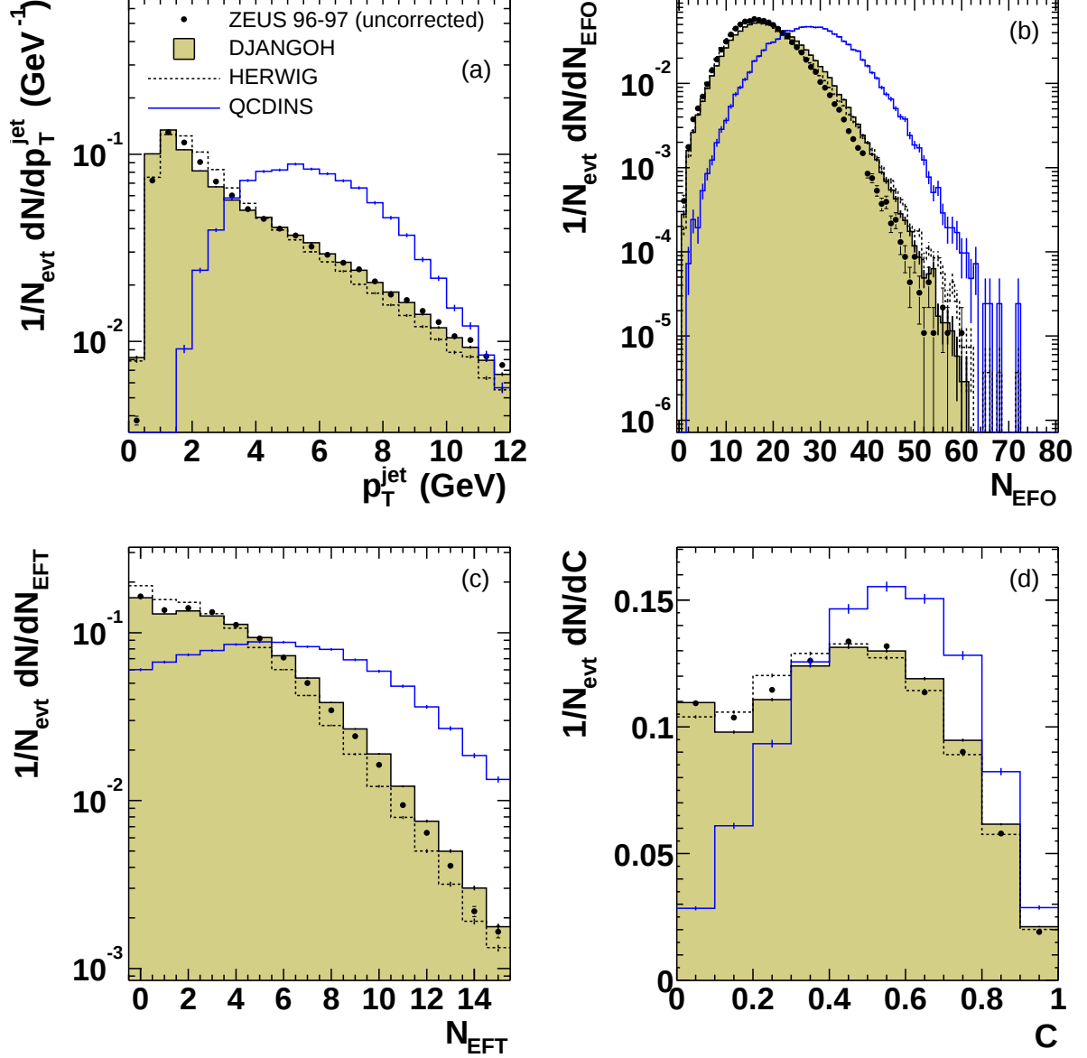
Figure 3: Distributions of variables calculated from the instanton region, shown for the fiducial sample: (a) the transverse momentum, p_T^{\text{jet}} , of the current jet, (b) EFO multiplicity, N_{\text{EFO}} , (c) EFO track multiplicity, N_{\text{EFT}} , (d) circularity, C , in the hcms. Statistical errors are given.
