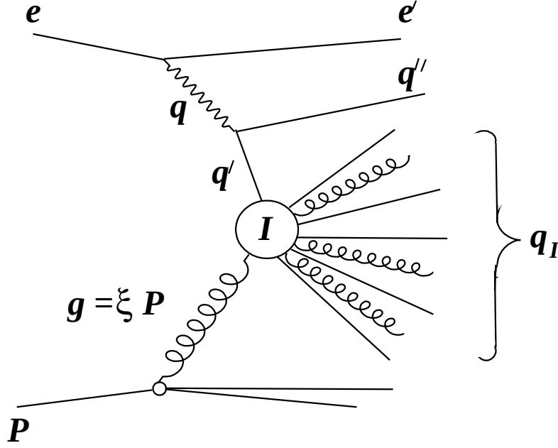
Figure 1: Kinematics of instanton-induced ep collisions.
