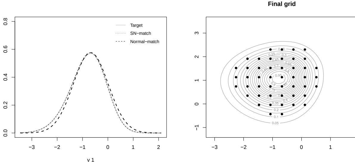
Figure 1: Left: Skew-normal fit (dotted) and naive Gaussian match (dashed) to the conditional \tilde{p}(v_1|\hat{v}_2, \mathcal{D}) (gray). The skew-normal fit is closer to the target and captures the lack of symmetry present in the target. Right: Final grid construction to explore \tilde{p}(\mathbf{v}|\mathcal{D}) .
