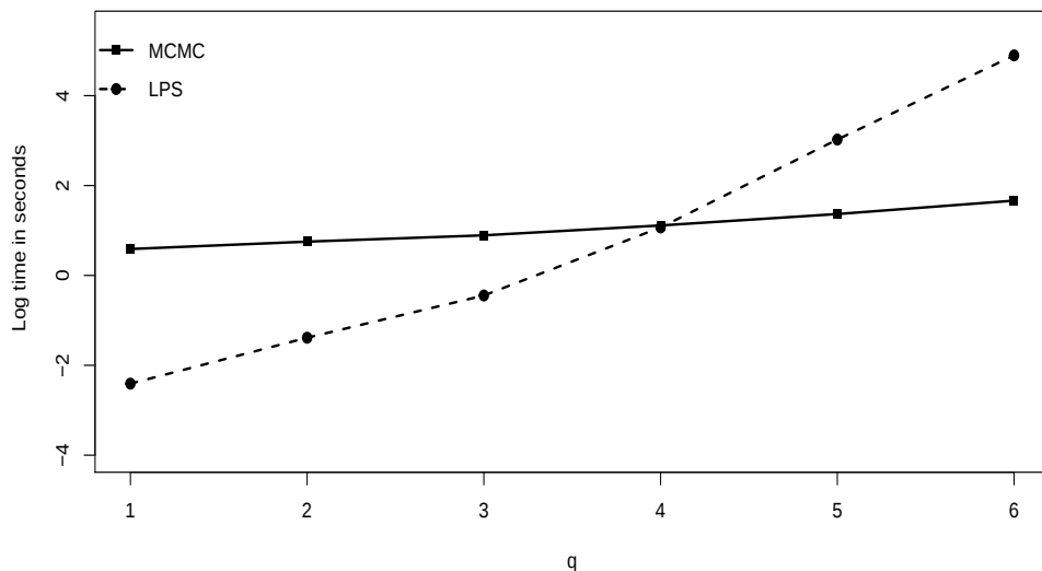
Figure 5: Logarithm of the average computation time (in seconds) of LPS (dashed) and LPS-MCMC (solid) over S = 20 samples of size n = 300 and dimensions q \in \{1, 2, 3, 4, 5, 6\} .
