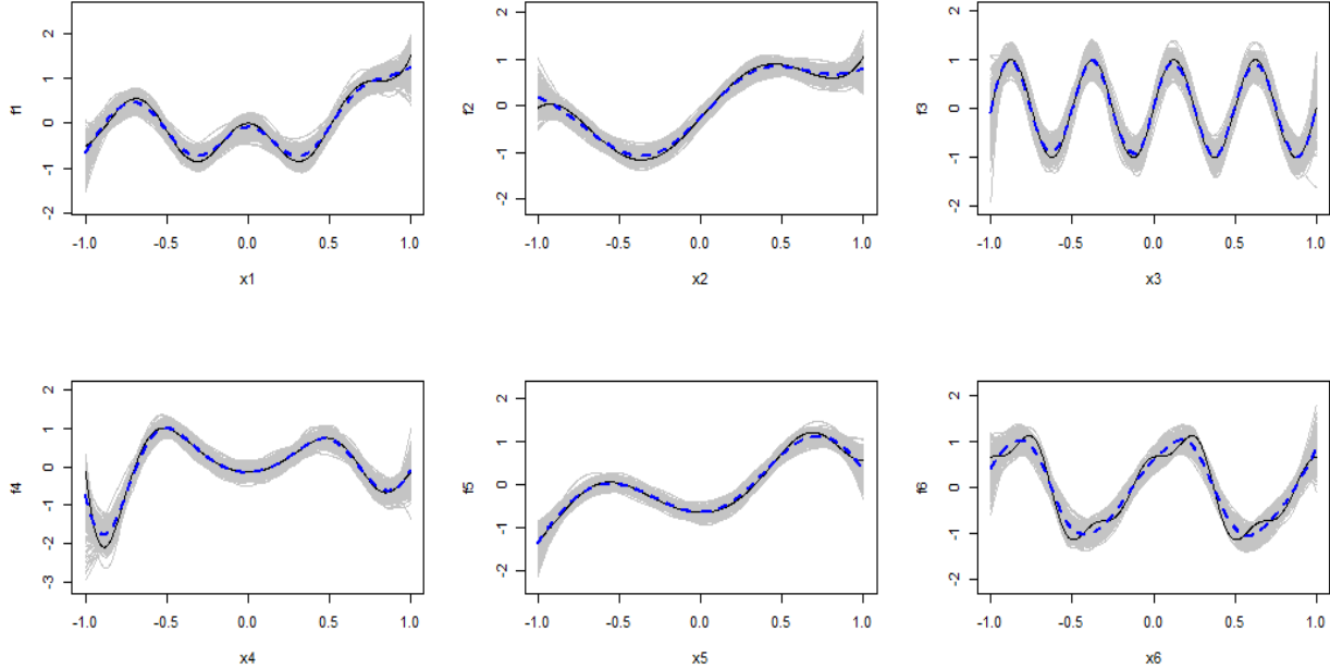
Figure 4: Estimation of smooth additive terms f_1, \dots, f_6 (gray curves) for S = 500 dataset replications of size n = 300 in the Binomial scenario. The dashed line is the pointwise median of the gray curves.
