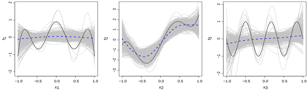
Figure 2: Estimation of smooth additive terms (gray curves) for S = 500 dataset replications of size n = 300 in the Bernoulli scenario with LPS. The dashed line is the pointwise median of the gray curves and the black curves are the target functions.
