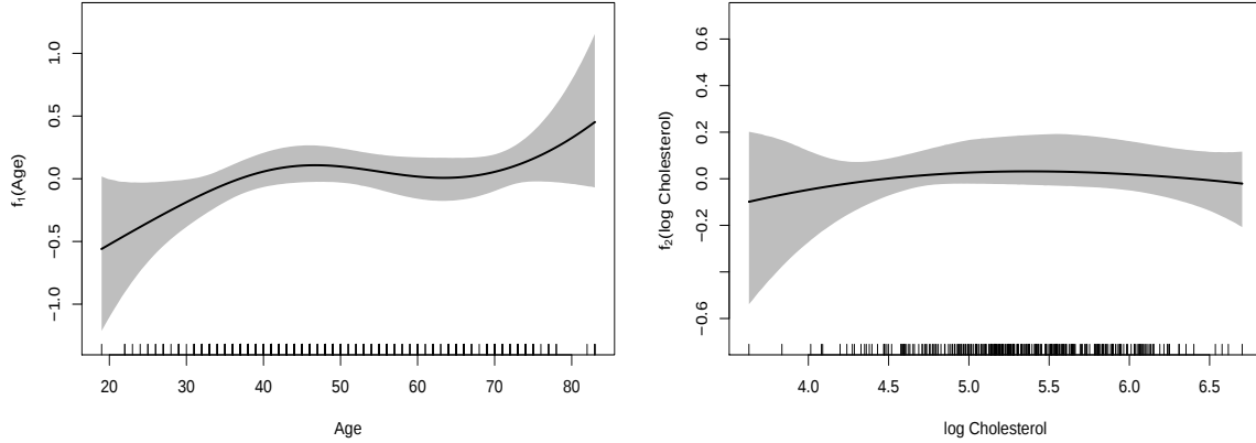
Figure 7: Estimated smooth functions (solid curve) and 95% approximate pointwise credible intervals (gray surface) for variables Age and \log(\text{Cholesterol}) of the nutritional study dataset.
