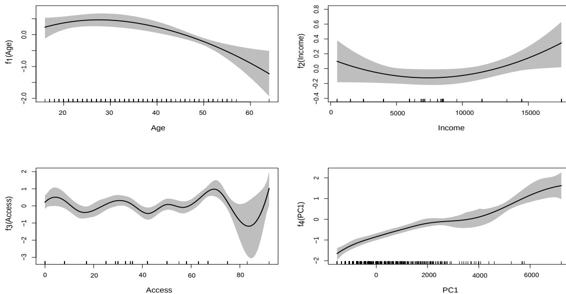
Figure 6: Estimated smooth functions (solid curve) and 95% approximate pointwise credible intervals (gray surface) for variables Age , Income , Access and PC1 .
