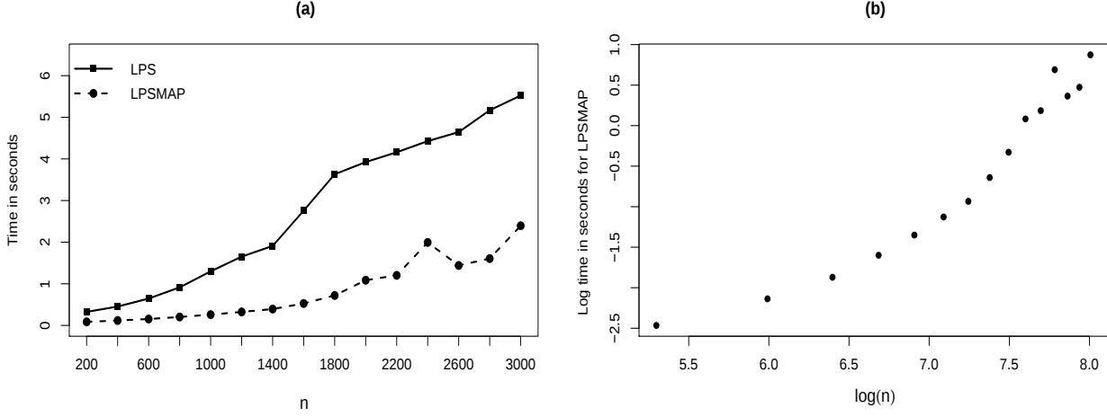
Figure 3: (a) Real elapsed time in seconds as a function of sample size for LPS and LPSMAP. (b) Computational time of LPSMAP against sample size on a log-log scale.
