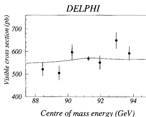
Fig. 3. Visible cross section of selected events as a function of centre of mass energy
