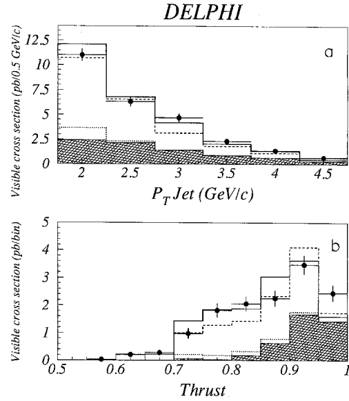
Fig. 8. Transverse momentum of jets (a) and the event thrust (b) for sample II in comparison with Monte Carlo predictions. QPM - hatched area, QPM+VDM - dots, QPM+VDM+GS ( p_T^{\min} = 1.83 GeV/c) - full line and QPM+VDM+LAC1 ( p_T^{\min} = 2.22 GeV/c) - dashed line
