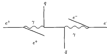
b) Direct photon contribution (QPM)
