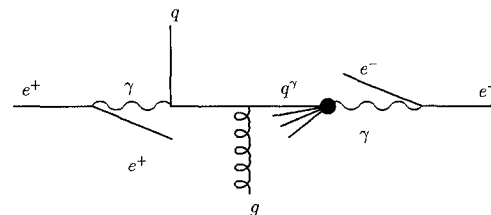
c) QCD singly resolved photon contribution
