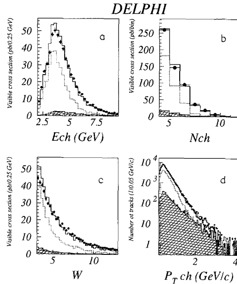
Fig. 5a-d. Distributions of event variables for sample I in comparison with Monte Carlo predictions. QPM - hatched area, QPM + VDM - dots, QPM + VDM + GS ( p_T^{\min} = 1.83 GeV/c) - full line. a Total energy of charged particles, b charged multiplicity, c invariant mass of the \gamma\gamma system and d transverse track momentum
