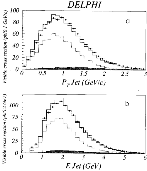
Fig. 6. Transverse momentum (a) and energy of the reconstructed jets (b) for sample I in comparison with Monte Carlo predictions. QPM - hatched area, QPM+VDM - dots, QPM+VDM+GS ( p_T^{\min} = 1.83 GeV/c) - full line
