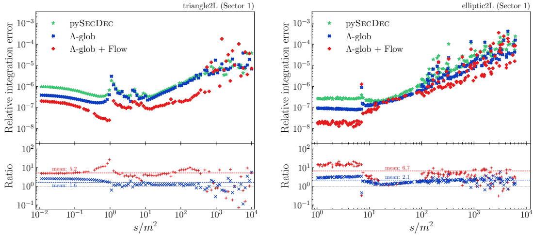
Figure 4: Relative integration error for sector one of a 2-loop triangle integral (left) and a 2-loop box integral known to contain elliptic functions (right) using the standard pySECDDEC algorithm (green), the ML-assisted \Lambda -glob algorithm (blue) and including an additional normalizing flow (red). The lower panel shows the ratios to the standard method. The figures are taken from Ref. [35].
