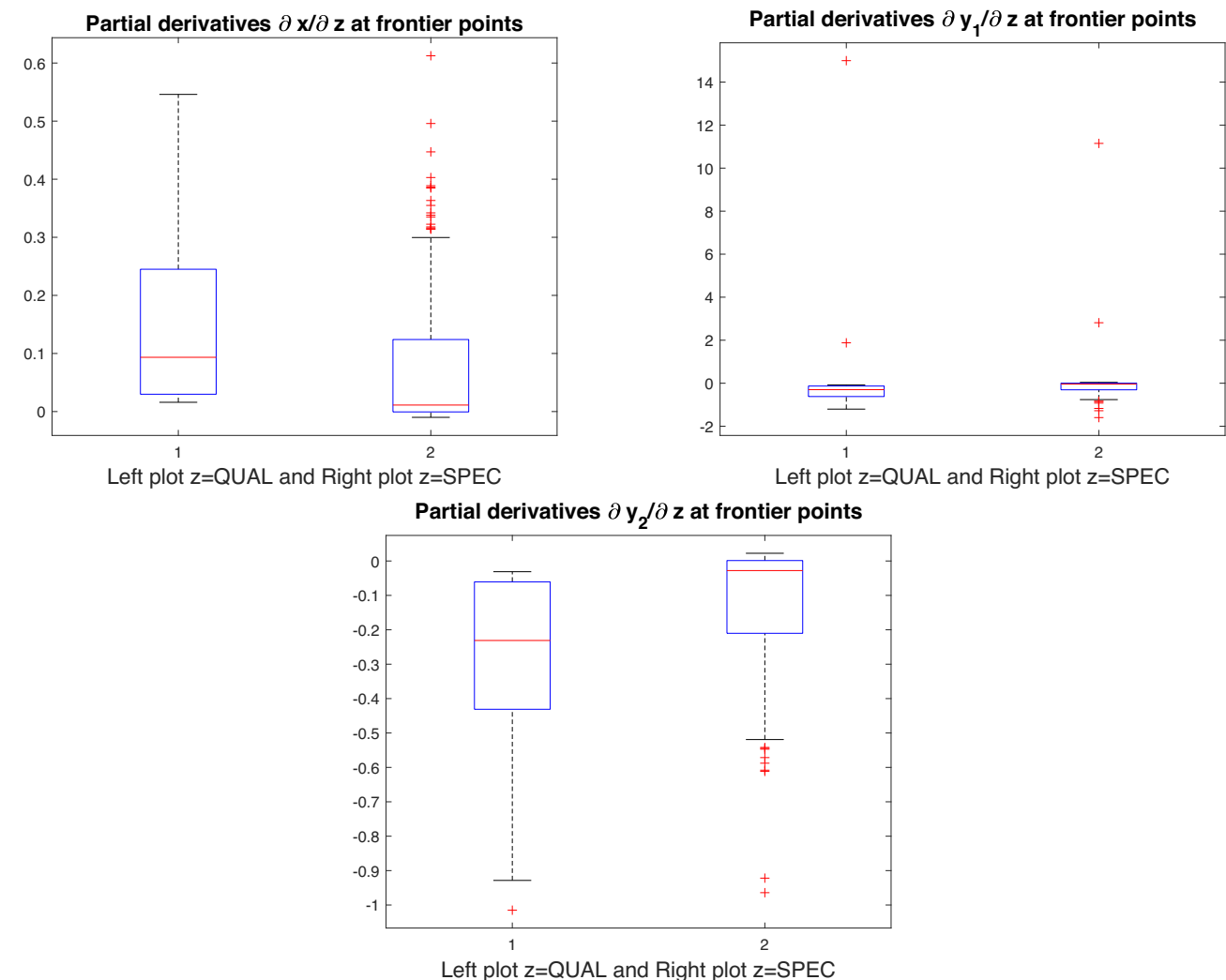
Fig. 5 HEI data: From left to right, plots of the estimated derivatives of \partial x/\partial z , \partial y_1/\partial z and \partial y_2/\partial z (in each plot, left case z_1 = QUAL and right case z_2 = SPEC )
