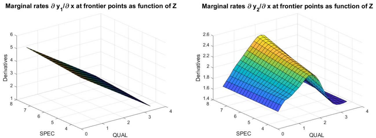
Fig. 6 HEI data: Local linear fit of the estimated derivatives of \partial y/\partial x , as a function of z , left panel y_1 and right panel y_2
