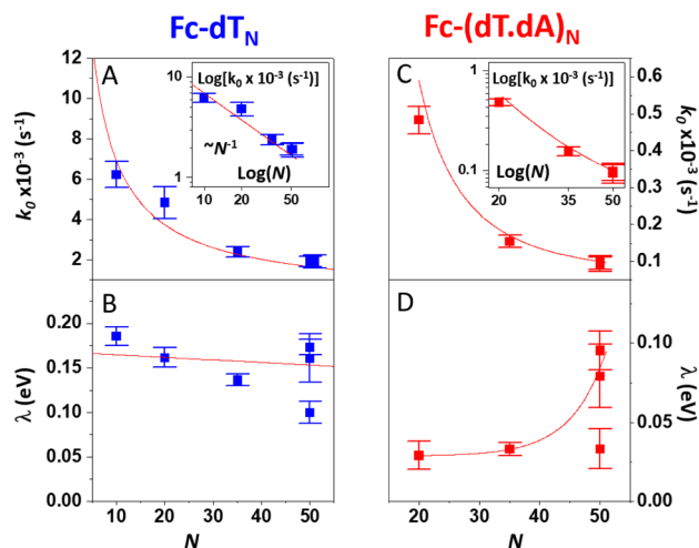
Fig. 4 Variation of the kinetic parameters k_0 and \lambda with the DNA chain length with various number of nucleotides ( N ). (A and B) Fc- \text{dT}_N . (C and D) Fc-( \text{dT.dA} ) _N . Red curves in (A) and (C), and insets are fits of eqn (2) to the data, in (B) and (D) are guides to the eye.
