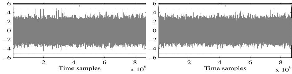
Fig. 5: T-test evaluation. C, no flags, d = 2 , secure routine for multiplication in GF(2^8) . Left: fresh randomness, 10k traces. Right: recycled randomness, 10k traces. No evidence of first-order leakage.
