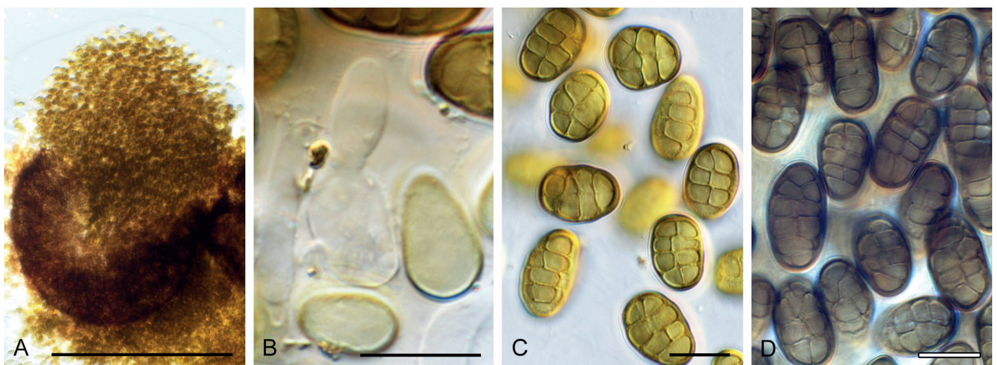
Fig. 33. Neocamarosporium leipoldiae (CPC 38543). A. Conidioma on SNA. B. Conidiogenous cell giving rise to conidia. C–D. Conidia. Scale bars: A = 300 µm, all others = 10 µm.
