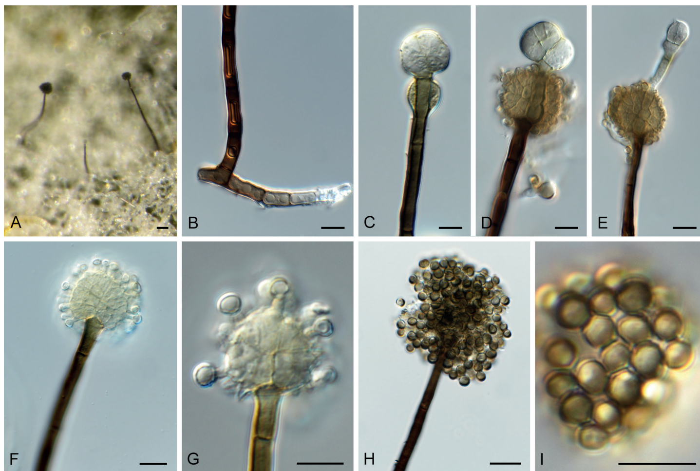
Fig. 74. Tryssglobulus aspergilloides (CPC 40100). A. Conidiophores in vivo. B. Base of conidiophore. C–E. Developing conidiophores with proliferation. F, G. Conidiogenous apparatus showing conidiogenesis. H. Conidiophore head with mature conidia. I. Conidia. Scale bars: A = 80 \mu m, all others = 10 \mu m.
