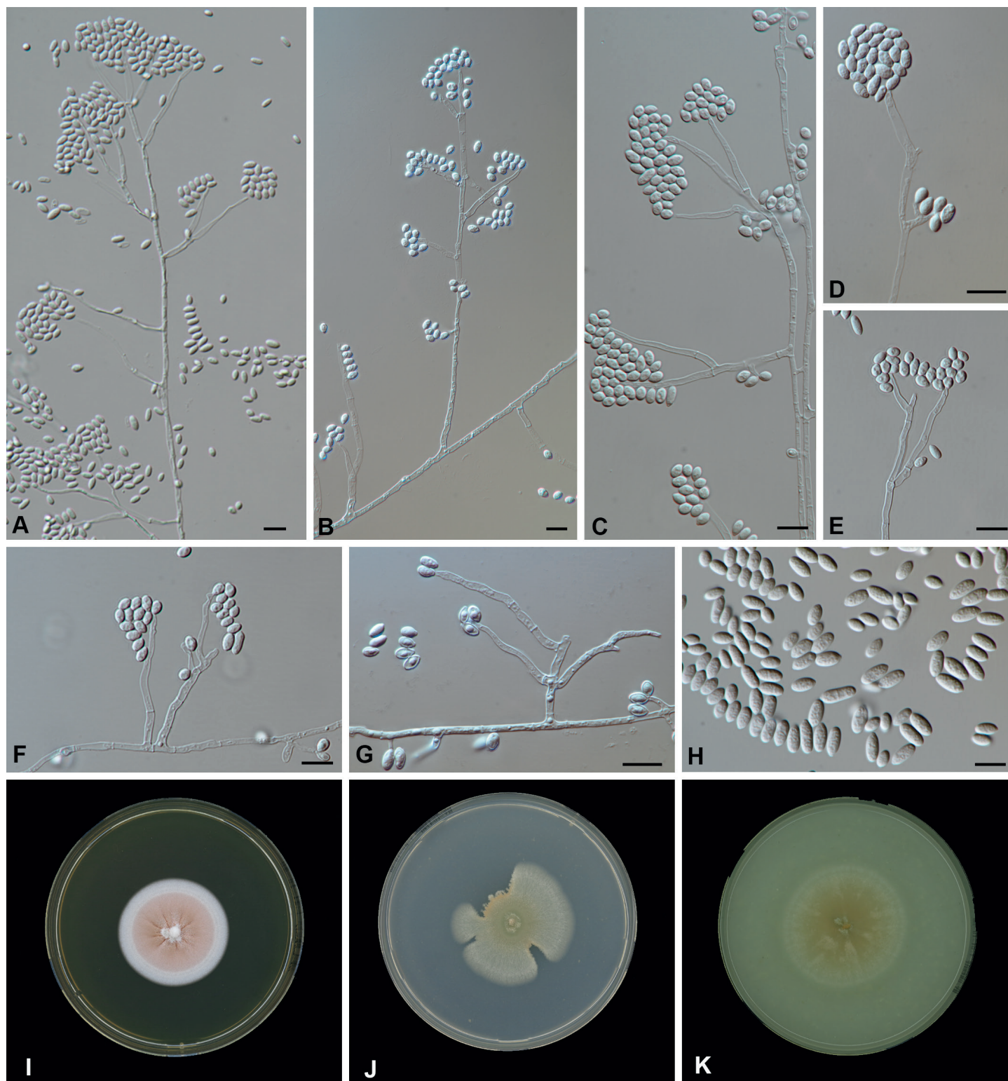
Fig. 51. Parasarocladium wereldwijsianum (CBS 147223). A–G. Conidiophores and conidia. H. Conidia. I. Colony on MEA. J. Colony on PDA. K. Colony on OA. Scale bars A–H = 10 \mu m.
