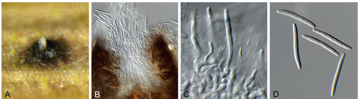
Fig. 29. Haudseptoria typhae (CPC 38203). A. Conidioma on host tissue. B. Conidiomatal ostiole. C. Conidiogenous cells giving rise to conidia. D. Conidia. Scale bars: A = 150 µm, all others = 10 µm.
