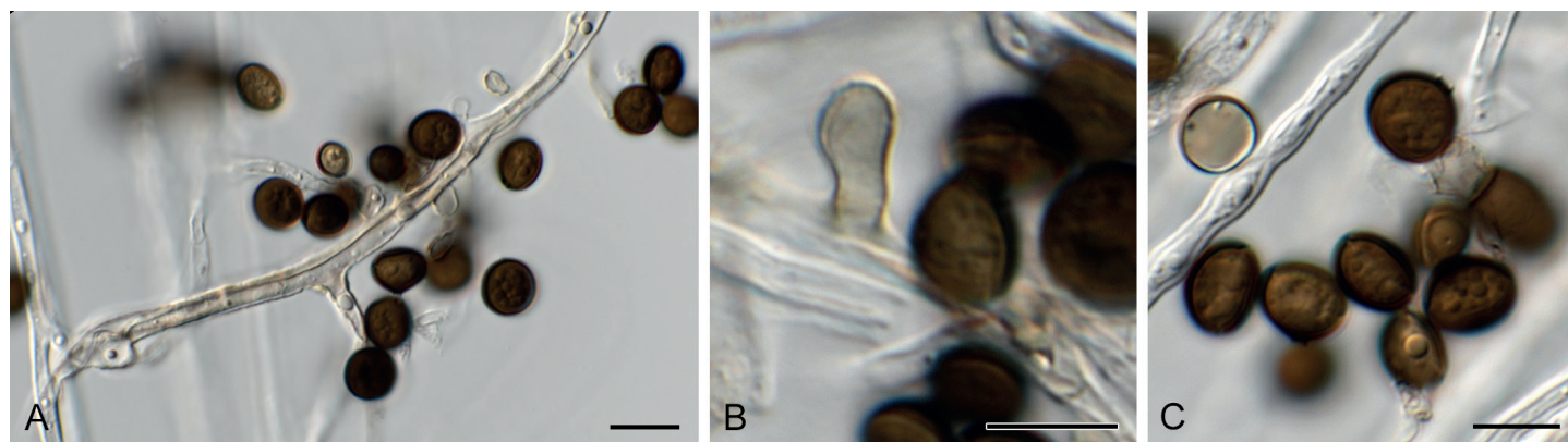
Fig. 11. Apiospora stipae (CPC 38101). A. Hyphae giving rise to conidiogenous cells with conidia. B–C. Conidiogenous cells and conidia. Scale bars = 10 µm.
