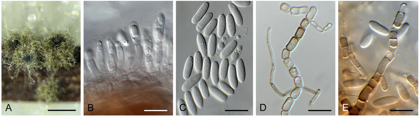
Fig. 39. Neoscytalidium dimidiatum (CPC 38666). A. Conidiomata on PNA. B. Conidiogenous cells. C. Fusicoccum-like conidia. D–E. Phragmoconidia, with a few fusicoccum-like conidia. Scale bars = 10 µm.
