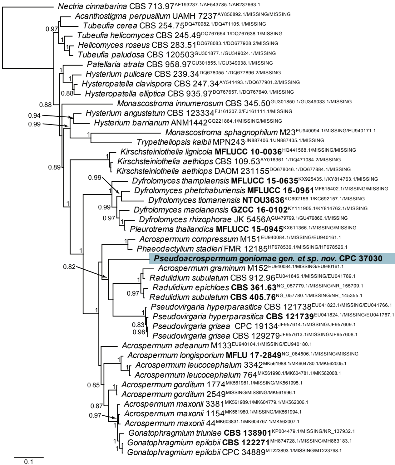
Fig. 62. Consensus phylogram (50 % majority rule) resulting from a Bayesian analysis of the Acrosporum and related genera multigene (LSU / tef1 / ITS) nucleotide alignment. The alignment is derived from Hudson et al. (2019). Bayesian posterior probabilities (> 0.79) are shown at the nodes and the scale bar represents the expected changes per site. GenBank accession (superscript) and / or culture collection / voucher numbers (in bold face when having a type status) are indicated for all species. The tree was rooted to Nectria cinnabarina (culture CBS 713.97) and the novel species treated in this study is indicated in a coloured block and bold face. Alignment statistics: 47 strains including the outgroup; 595 / 418 / 284 unique site patterns, respectively. Tree statistics: 184 502 sampled trees from 1 230 000 generations.
