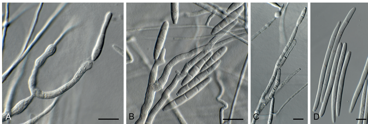
Fig. 25. Flammocladia anomiae (CPC 36302). A–C. Conidiogenous cells giving rise to conidia. D. Conidia. Scale bars = 10 \mu m.
