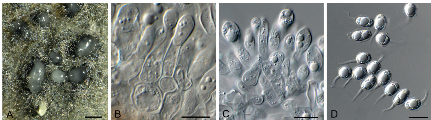
Fig. 55. Phyllosticta phoenicis (CPC 39164). A. Colony sporulating on OA. B–C. Conidiogenous cells. D. Conidia. Scale bars: A = 250 µm, all others = 10 µm.
