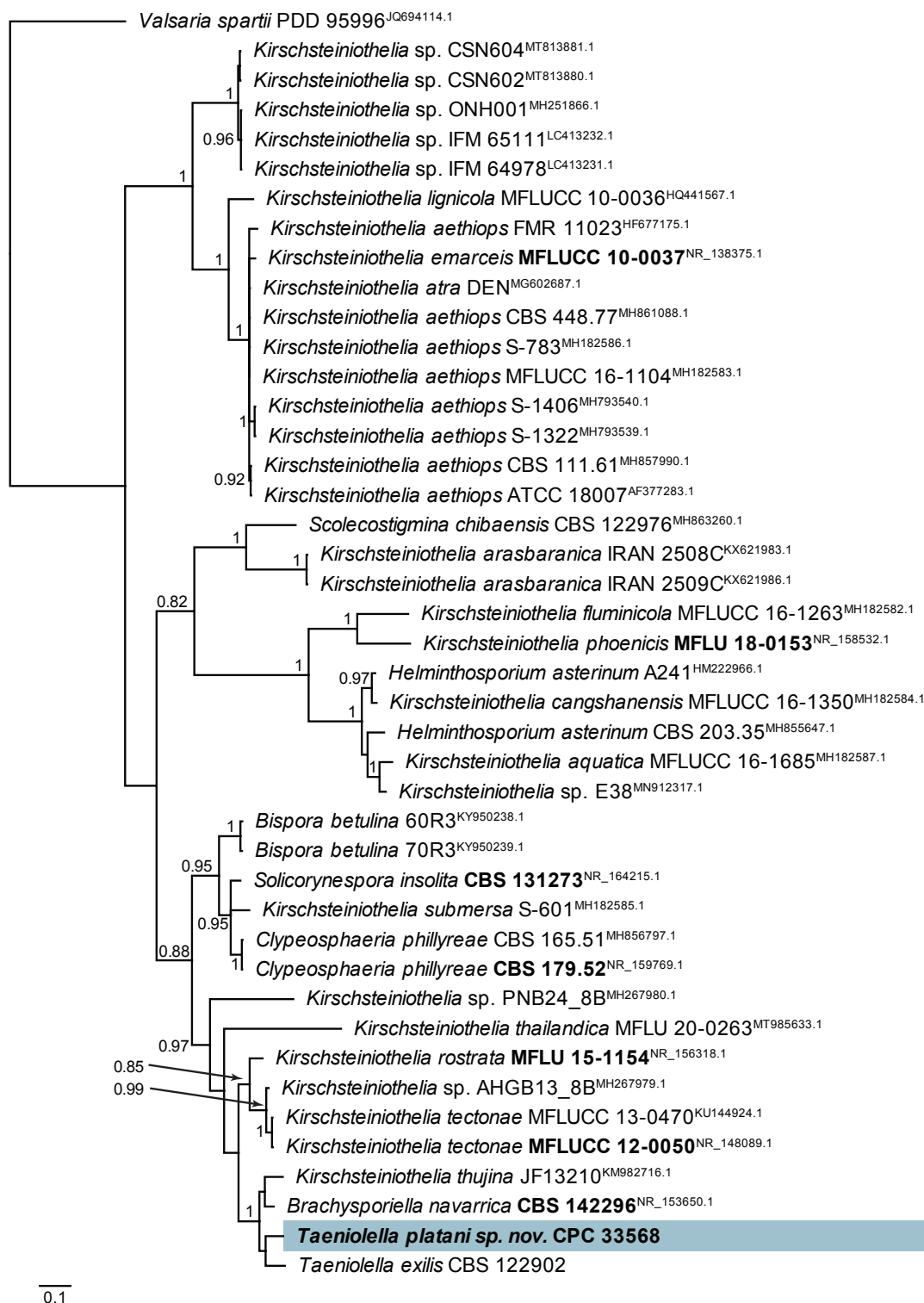
Fig. 72. Consensus phylogram (50 % majority rule) resulting from a Bayesian analysis of the Kirschsteiniethelia s. lat. ITS nucleotide alignment. Bayesian posterior probabilities (> 0.79) are shown at the nodes and the scale bar represents the expected changes per site. GenBank accession (superscript) and / or culture collection / voucher numbers (in bold face when having a type status) are indicated for all species. The tree was rooted to Valsaria spartii (voucher PDD 95996; GenBank JQ694114.1) and the novel species treated in this study is indicated in a coloured box and bold face. GTR + I + gamma and dirichlet frequencies were used as substitution model. Alignment statistics: 43 strains including the outgroup. Tree statistics: 382 unique site patterns; 4 502 sampled trees from 15 000 generations.
