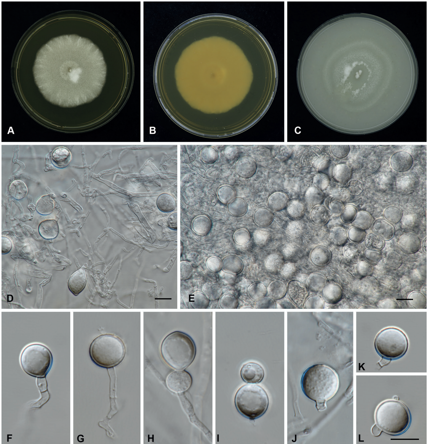
Fig. 31. Hogelandia lambearum (CBS 147626). A–B. Colony on MEA. C. Colony on OA. D–E. Mycelium and conidia. F–H. Conidiogenous cells and conidia. I–L. Conidia. Scale bars D–E, L = 10 µm. L applies to F–L.
