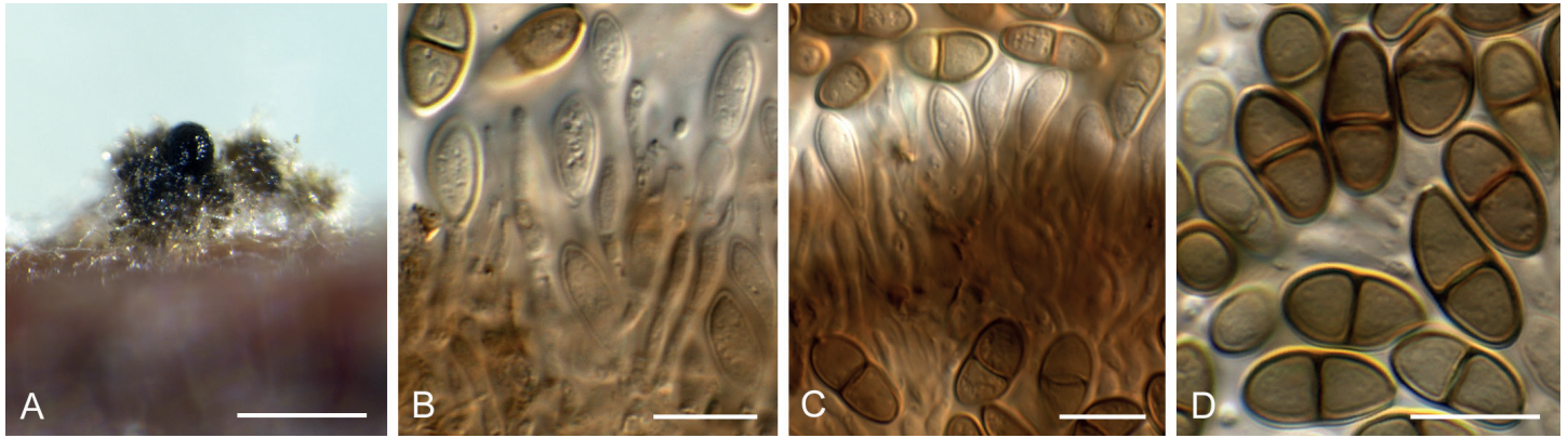
Fig. 60. Porodiplotidia vitis (CPC 38692). A. Conidiomata on PNA. B–C. Conidiogenous cells. D. Conidia. Scale bars: A = 300 \mu m, all others = 10 \mu m.
