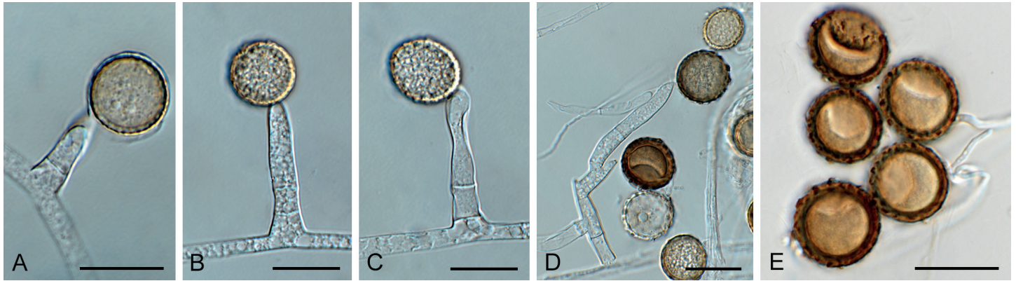
Fig. 28. Harzia tenella (CPC 38667). A–D. Conidiogenous cells giving rise to conidia. E. Conidia. Scale bars = 10 µm.
