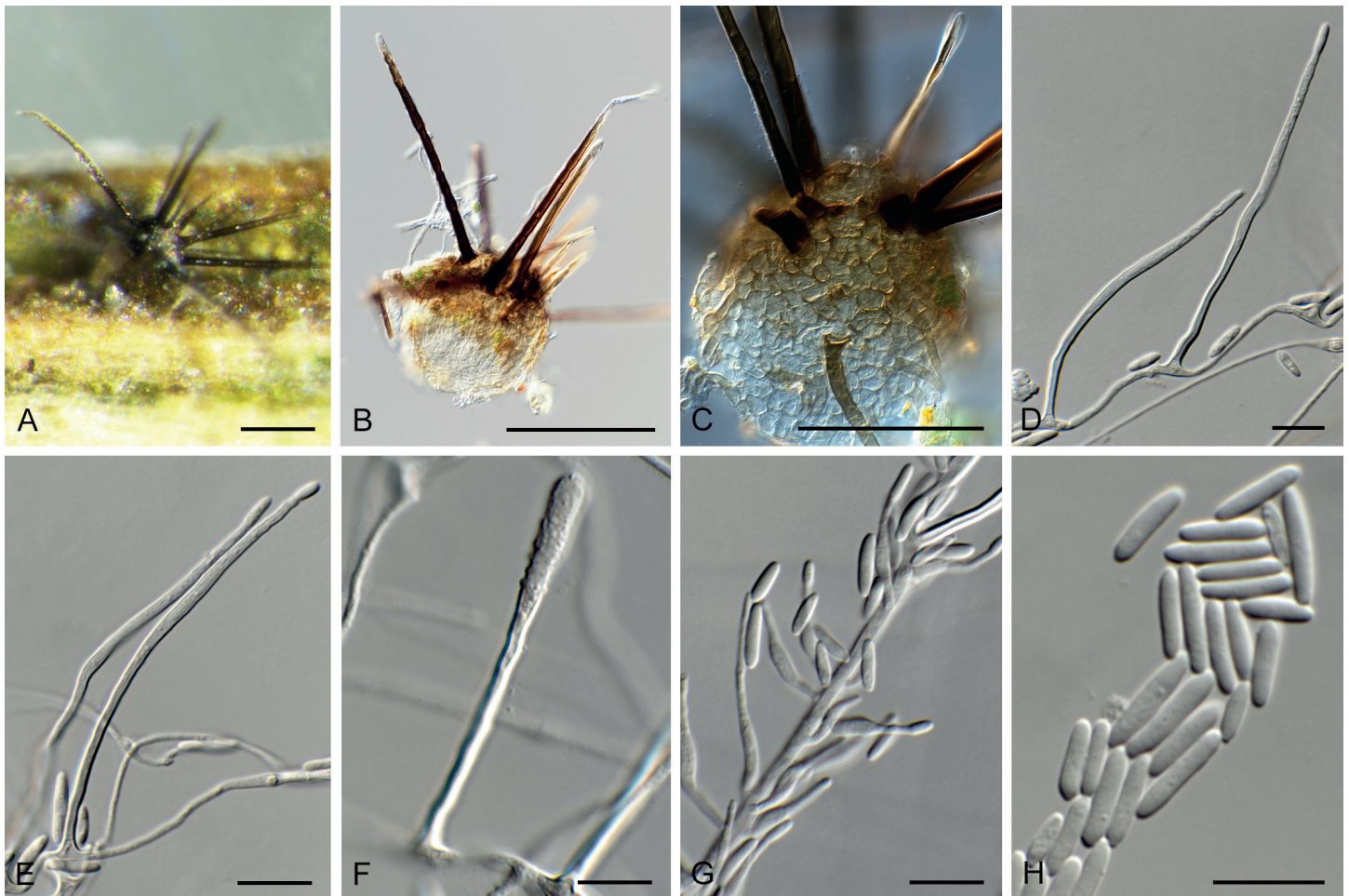
Fig. 40. Niesslia neoexosporioides (CPC 38177). A. Ascoma on host tissue. B–C. Ascomata with setae. D–F. Stipes with clavate vesicles. G. Conidiogenous cells. H. Conidia. Scale bars: A–B = 100 µm, C = 50 µm, all others = 10 µm.
