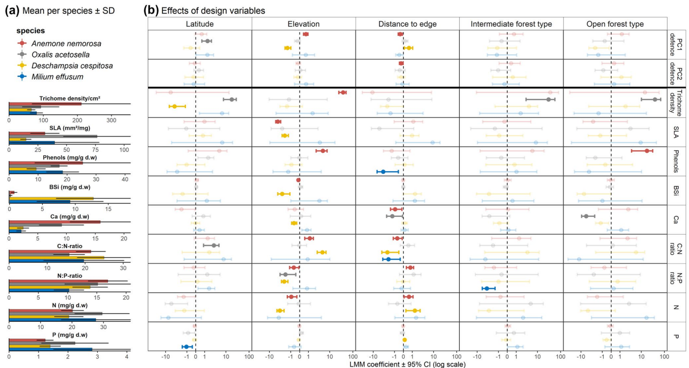
FIGURE 2 (a) Mean of plant trait values per species \pm standard deviation (SD) across 15 geographic sites in Europe. Chemical plant traits are expressed per mass dry weight (d.w.). (b) Log transformed linear mixed effect model (LMM) coefficient estimates [ \pm 95% confidence intervals (CI)] for latitude, elevation, distance to the forest edge and forest management type on two multivariate defence phenotypes [ PC1_{DEFENCE} and PC2_{DEFENCE} ], and on trichome density, specific leaf area (SLA), biogenic silica concentration (BSi), total phenolic concentration (phenols), calcium concentration (Ca), carbon : nitrogen (C : N ratio), nitrogen : phosphorus (N : P ratio), nitrogen concentration (N) and phosphorus concentration (P). The effects of 'Intermediate forest type' and 'Open forest type' are expressed relative to 'Dense forest type'. Significant effects ( p < .05 ) are plotted in bold. Non-significant effects ( p \geq .05 ) are faded
