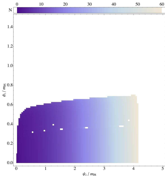
FIG. 8: Grid of initial conditions, for hybrid potential with M = 0.03m_{\text{pl}} , m = 10^{-6}m_{\text{pl}} , \lambda = 1 , \lambda' = 0.1 .
