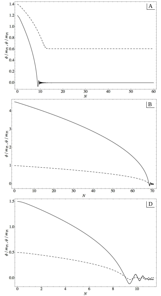
FIG. 5: Evolution of the fields \phi (dashed lines) and \psi (plain lines) with the number of e-folds realized, for the trajectories A, B, and D (from top to bottom) as represented in Fig. 4. The more interesting type-C trajectory is represented in Fig. 6 below.
