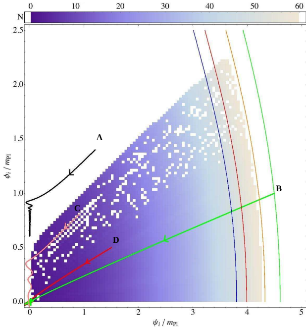
FIG. 4: Grid of initial conditions leading to successful (white regions) and unsuccessful inflation (colored region), for the original hybrid inflation with \lambda = \lambda' = 1 , m = 10^{-6}m_{\text{pl}} and M = 0.03m_{\text{pl}} . The color code denotes the number of e-folds realized. Three typical successful trajectories [in the valley (A), radial (B), and from an isolated point (C)] are added as well as an unsuccessful trajectory (point D). Also plotted are the iso-curves of \epsilon_1 , in the slow-roll approximation, for \epsilon_1 = 0.022, 0.02, 0.0167 and 0.015 (from left to right).
