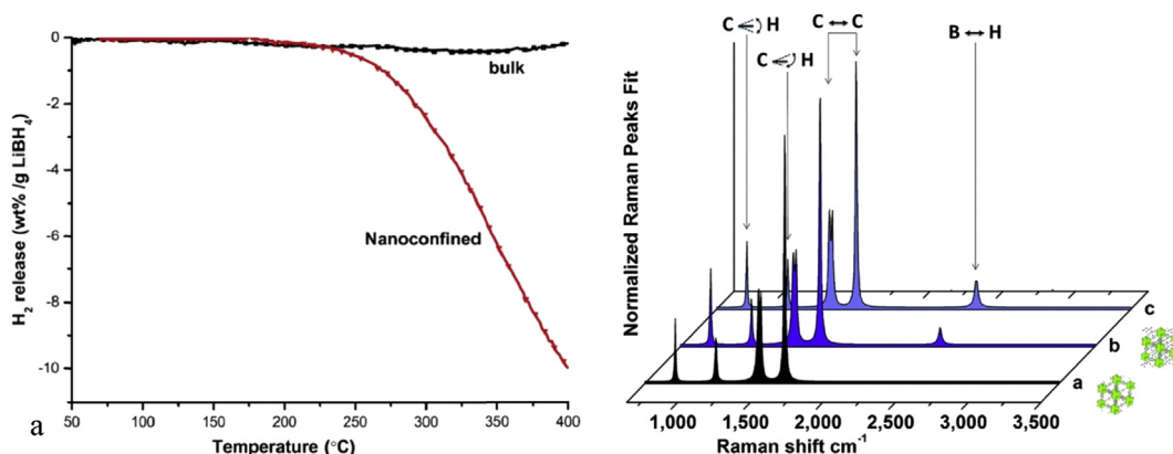
Fig. 2 – Two examples of how nanoconfinement can change the stability of complex metal hydride materials. (a, left) \text{H}_2 release from macrocrystalline \text{LiBH}_4 and from \text{LiBH}_4 confined in a nanoporous carbon scaffold, measured at p(\text{H}_2) = 1.1 bar \text{H}_2 and heating with 3^\circ\text{C}/\text{min} , showing how nanoconfinement destabilizes and lowers the 410^\circ\text{C} equilibrium temperature under 1 bar \text{H}_2 with \sim 150^\circ\text{C} [137]; (b, right) Raman spectra showing how the normally at room temperature unstable \text{Ti}(\text{BH}_4)_3 is stabilized by confinement in a MOF, (a) empty MOF, (b) MOF loaded with \text{Ti}(\text{BH}_4)_3 , (c) the same sample after 1 months storage in Ar at RT [138].
