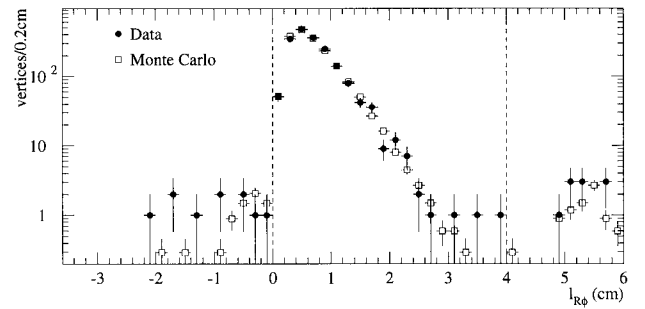
Fig. 3. The R\phi decay lengths of the accepted vertices in simulation and data. Negative lengths correspond to vertices which would have passed the \delta\phi cut had their momentum vector been reversed. The radius of the beam pipe was 5.5 cm
