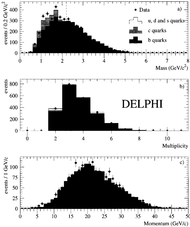
Fig. 2. a) The reconstructed masses of the vertices, b) the multiplicity of the secondary vertices, and c) the summed momenta at those vertices. Only the finally accepted events are shown, except that in a) and b) those rejected only by the relevant cut are also shown
