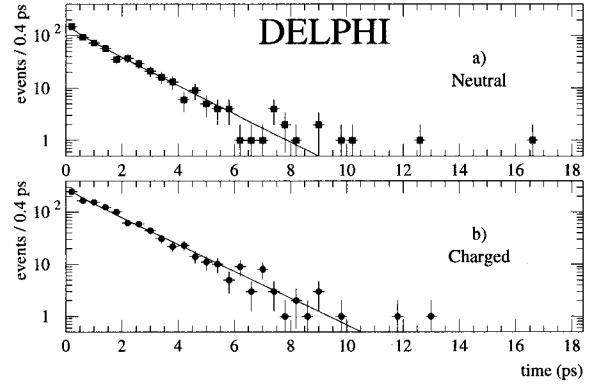
Fig. 6. The excess proper time distributions of the charged and neutral vertices, with the fit result superimposed. The slight curvature is because the fit is a sum of exponentials
