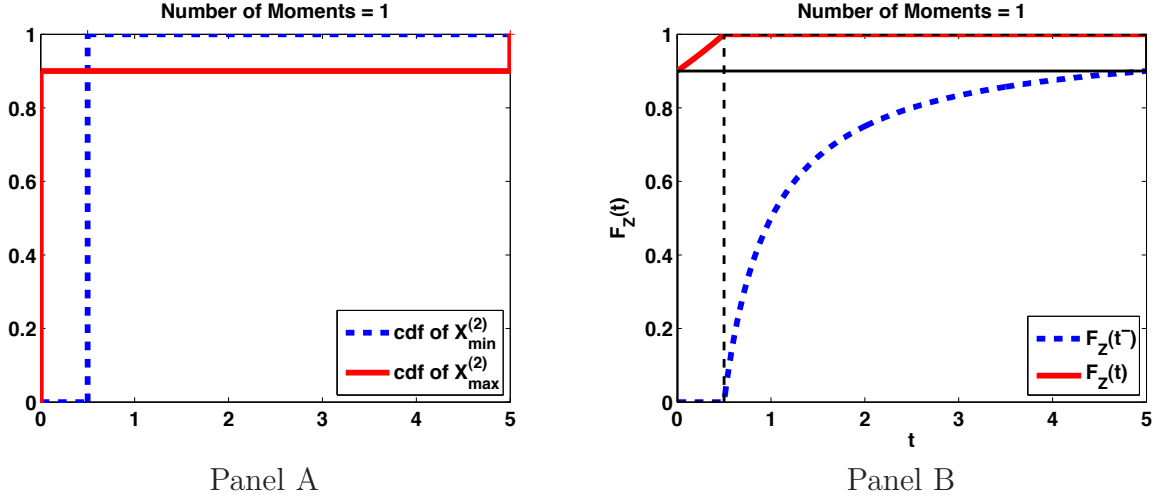
Figure 3.1: Case s = 2 , m = 1 : The left panel displays the extreme cdfs of X_{\min}^{(2)} and X_{\max}^{(2)} and the right panel draws F_Z(t) and F_Z(t^-) = P[Z < t] on top of these extreme cdfs with \mu_1 = \frac{1}{2} , a = 0 and b = 5 . Note that we omitted the indice in the notation of the random variable Z but for each t , the random variable Z depends on t . The curves represented in Panel B and denoted by abuse of notation F_Z(t) and F_Z(t^-) are F_{Z_t}(t) and F_{Z_t}(t^-) . The lower and upper curves in Panel B should be interpreted as bounds on the F_Z(t) when two moments are fixed.
