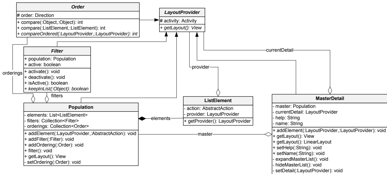
Figure 2. The UML Class Diagram of Mandroid.
