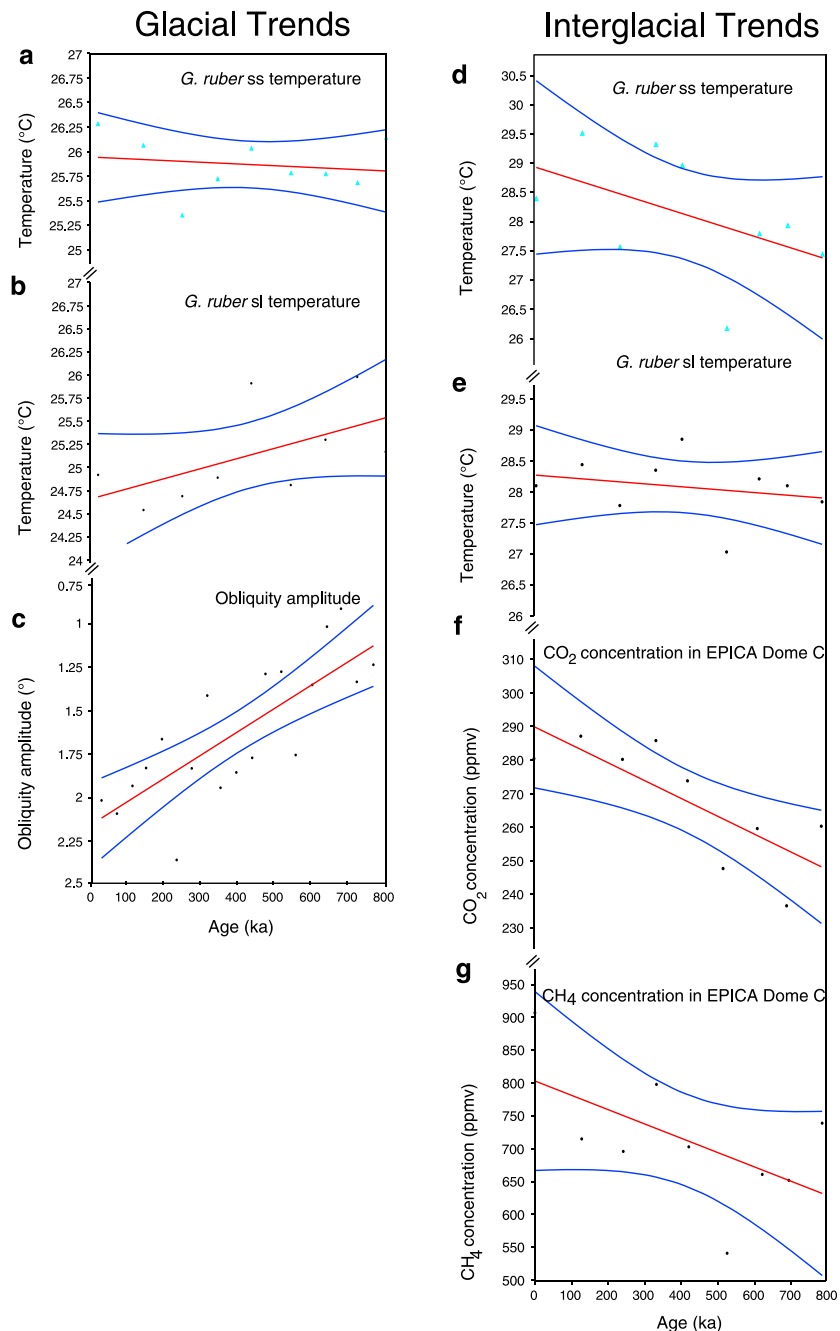
Figure 4. Long-term trends of paleoclimatic proxies: (a, b) glacial temperatures and (d, e) interglacial temperatures for G. ruber ss and G. ruber sl. Long-term trend of (c) obliquity angle [Mélis et al., 2001] and (f, g) EPICA DOME C records of CO 2 [Loulergue et al., 2008] and CH 4 [Lüthi et al., 2008]. Blue lines indicate the 95% confidence interval. Data and results of Student's t tests are available in Tables 1 and S2.
