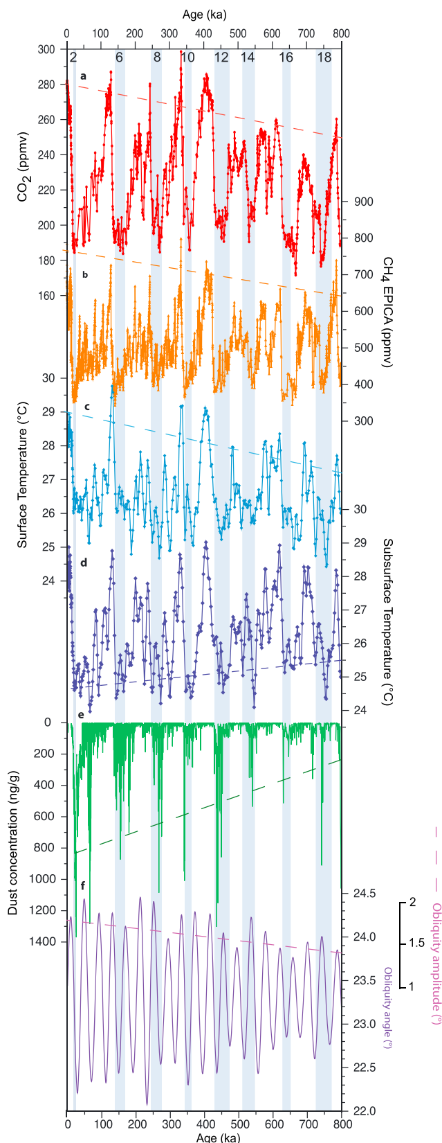
Figure 8. Long-term evolution of temperatures in the GoP compared to other paleoclimatic records. (a, b) CO 2 and CH 4 concentrations in EPICA Dome C core from Antarctica [Loulergue et al. , 2008; Lüthi et al. , 2008]. (c, d) Temperatures records of G. ruber ss (clear blue) and G. ruber sl (dark blue) of core MD05-2930. (e) Dust deposition record of EPICA Dome C of Antarctica [Lambert et al. , 2008]. (f) Obliquity angle and amplitude [Mélis et al. , 2001]. Dashed lines of Figures 8a–8c indicate long-term trends of interglacial mean values. Dashed lines of Figures 8d and 8e indicate long-term trend of glacial mean values. Dashed line of Figure 8f indicates evolution of obliquity amplitude through the last 800 ka. Gray bars and numbers indicate glacial stages. Statistical tests of long-term trend are indicated in Table S2.
