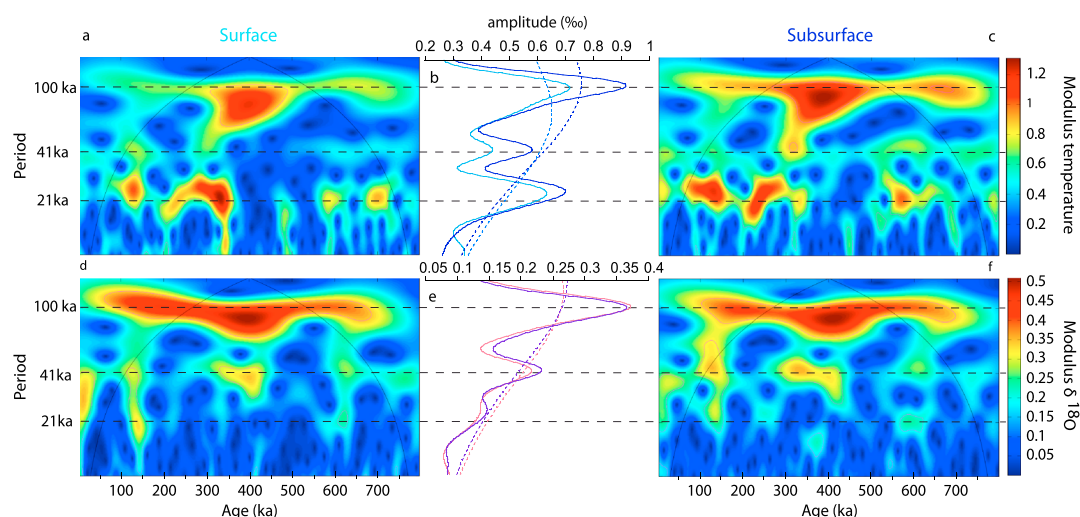
Figure 6. Time series analyses (modulus of the continuous wavelet transform) of (a, c) Mg/Ca-derived temperatures and (d, f) \delta^{18}\text{O}_{\text{calcite}} of surface ( G. ruber ss ) and subsurface ( G. ruber sl ) of core MD05-2930. Black lines delimit the cones of influence and pink contours enclose the \geq 95\% confidence areas for a red noise background hypothesis. (b, e) Square root of the global wavelet spectrum (solid lines) and 95% confidence level for a red noise background hypothesis (dashed lines) computed for the Mg/Ca-derived temperatures and \delta^{18}\text{O}_{\text{calcite}} (light colors for G. ruber ss and dark colors for G. ruber sl ).
