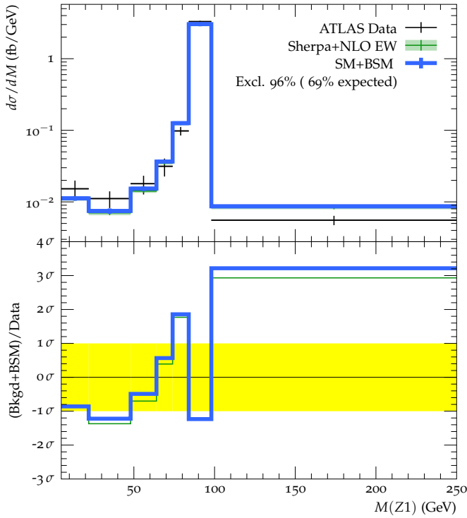
Figure 3: Upper panel: Representative differential cross section as a function of the highest-mass dilepton pair in 4\ell measurements used in this study showing ATLAS data (crosses) [79], predicted SM yields (green) [82], and predicted SM+BSM yields for (M_{\Delta^{++}}, M_{\Delta^+}) = (180 \text{ GeV}, 255 \text{ GeV}) (blue). Lower panel: bin-by-bin significance of expected theory yields relative to data with combined data and theory uncertainties (band).
