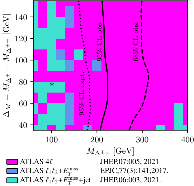
Figure 2: The (M_{\Delta^{++}}, \Delta_M) parameter space overlaid with the 95% (solid) and 68% (long-dash) exclusion limits as obtained from MadGraph5_aMC@NLO + Contur. (Values to the left of the lines are excluded.) Also shown is the 95% expected exclusion (dotted). The color-shading scheme indicates which SM measurement provides the dominant exclusion. The black asterisk indicates the best fit value from [22].
