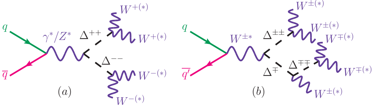
Figure 1: Graphs illustrating the production of Type II scalars in (a) neutral-current and (b) charged-current quark-antiquark annihilation at the Born level and their decays to W bosons. Drawn with JaxoDraw [66].
