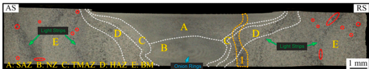
Figure 24. Macrography of FSW joint for the WAAM 205A fabricated sample [64].
