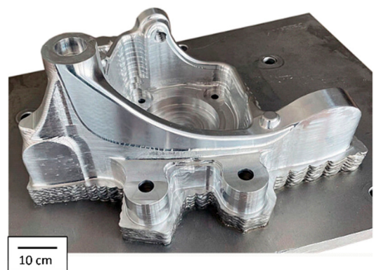
Figure 2. Aluminium parts manufactured by PBF-LB (a) and WAAM (b) processes. At the left, ER 2024 and ER 6061 aluminium parts manufactured by Elementum 3D (adapted from [10]). At the right, an ER 5183 aluminium part manufactured by Migal (adapted from [11]).
