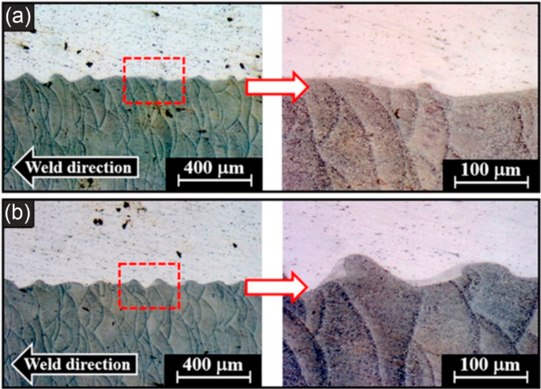
Figure 26. Macrography in the beginning region (a) and the centre region (b) of the MPW joint of PBF-LB AlSi10Mg fabricated sample. The last one (b) shows the formation of “regular” waves, slightly larger “peak-to-peak” than the beginning region of the weld seam.(adapted from [73]).
