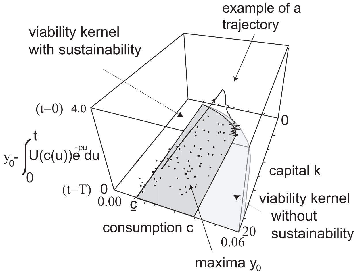
Figure 4: Maximal \int_0^T w(c(\tau)) e^{-\rho \tau} d\tau with (k(\cdot), c(\cdot), t(\cdot), V(\cdot)) remaining in the set of constraints, and particular trajectory leading to maximal \int_0^T w(c(\tau)) e^{-\rho \tau} d\tau with (k(\cdot), c(\cdot), t(\cdot), V(\cdot)) remaining in the set of constraints. Case f(k) = 0.04\sqrt{k} , n + \delta = 0.01 , \rho = 0.05 , \sigma = 0.5 .
