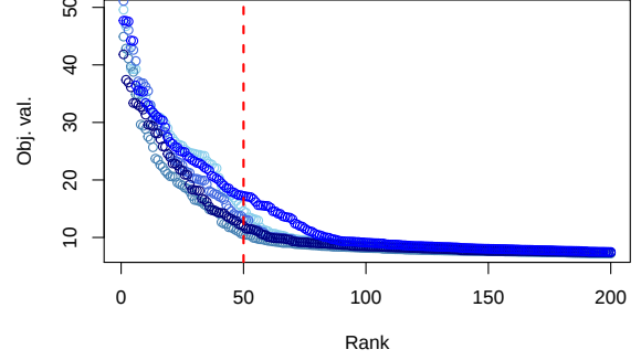
(b) 5 runs of the Jurkat vs 293T experiment with 10 rare cells among total of 1,000 cells ( \kappa = 0.1 ).
