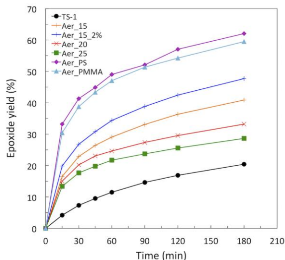
Figure 8. Kinetic data in terms of epoxide yield for the reaction of cyclohexene with cumene hydroperoxide (CHP) in toluene. Experimental conditions: T = 90^\circ\text{C} , [CATA] = 5 \text{ g} \cdot \text{l}^{-1} , [Cyclohexene] = 0.9 \text{ mol} \cdot \text{l}^{-1} , [CHP] = 0.18 \text{ mol} \cdot \text{l}^{-1} .
