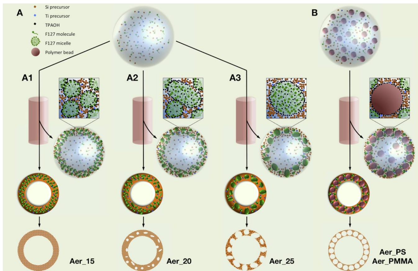
Figure 2. Schematic representation of the routes used for the preparation of \text{TiO}_2\text{-SiO}_2 with tailored porosity. In “Route A”, the porosity was controlled by increasing the TPAOH to (Si+Ti) molar ratio, which allows to move from a mesoporous material formed by an evaporation-induced self-assembly mechanism (Route A1) to a macroporous solid resulting from a phase separation mechanism (Routes A2 and A3). In “Route B”, macropores were generated by a hard-templating approach using polymer beads of various sizes.
