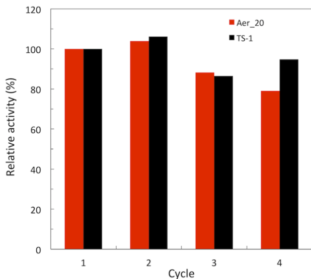
Figure 9. Recyclability study of the TS-1 and Aer_20 catalysts with CHP as oxidant. Data were collected in the initial stage of the reaction (15 min reaction time) and the catalytic activity (expressed in terms of CHP conversion) relative to the first test was calculated for each catalyst. The composition was identical to Figure 8 .
