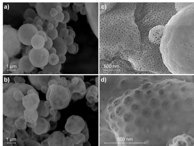
Figure 5. SEM (a–b) and SEM-FEG (c–d) images of Aer_PS (a, c) and Aer_PMMA (b, d). Additional SEM pictures can be found in the Supporting Information ( Figure S3 ).
