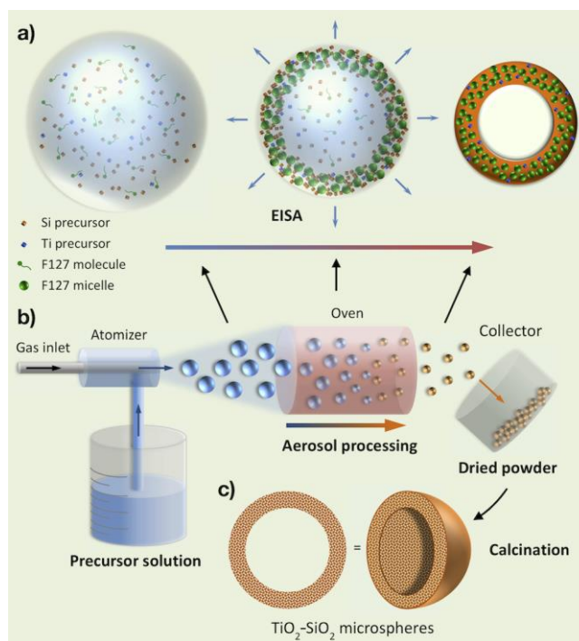
Figure 1. Preparation of mesostructured TiO 2 -SiO 2 microspheres by a so-called Type IIIc aerosol technique. 40 a) Illustration of the evaporation-induced self-assembly (EISA) mechanism (TPAOH has been omitted for clarity); b) Schematic representation of the aerosol set-up; c) Illustration of the texture and morphology of the calcined material in the typical conditions used (see the experimental section for further details).
