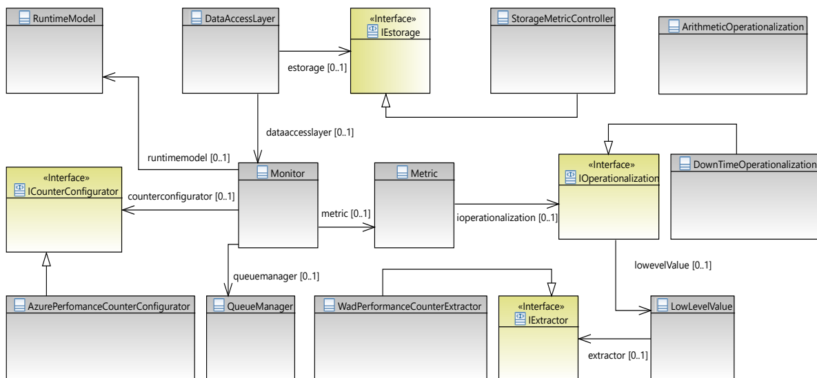
FIGURE 5. Middleware architecture for Microsoft Azure.
