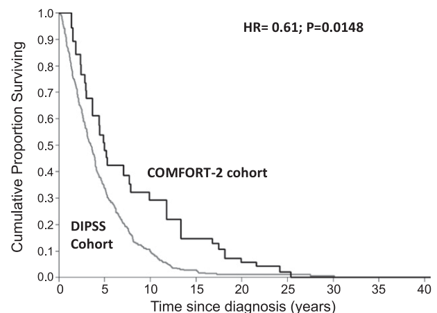
Figure 1. Survival estimate from diagnosis of PMF patients who become intermediate-2 and high risk IPSS with a blast cell count <10\% at any time of their follow-up according to the COMFORT-2 (n = 100) and DIPSS (N = 350) cohorts.
