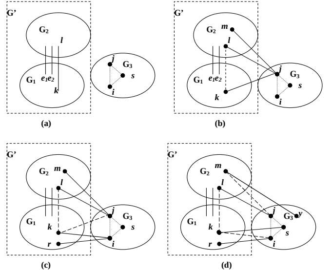
Fig. 3. Illustration of implementation of a meta-1-splitting operation in \mathbb{R}^2 : (a) before performing a meta-1-splitting (b) performing first HC operation to split an existing meta-edge (l, k) (c) performing second HC operation to split a newly added meta-edge (j, k) , obtaining a rigid meta-formation (d) performing additional HC operations to obtain meta-edges which do not incident on common agents
