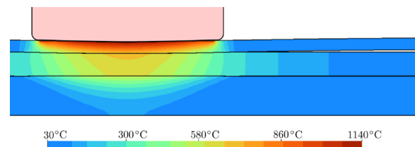
Fig. 13 Illustrative solution from a pure-FEM model of the FMB process. The three plates are modelled as deformable solids that can interact through a contact algorithm. Deformation through plate thickness and bending of the steel plate are observed. The displacements are magnified by a factor 10 for visualisation purposes
