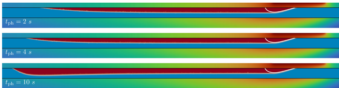
Fig. 14 Simulations for different preheating times ( t_{ph} ) but same tool temperature ( T_{tool} = 852^{\circ}\text{C} ) and travel speed ( v_{tool} = 200 \text{ mm/min} ). All the snapshots are taken at 24 s after starting the tool displacement
