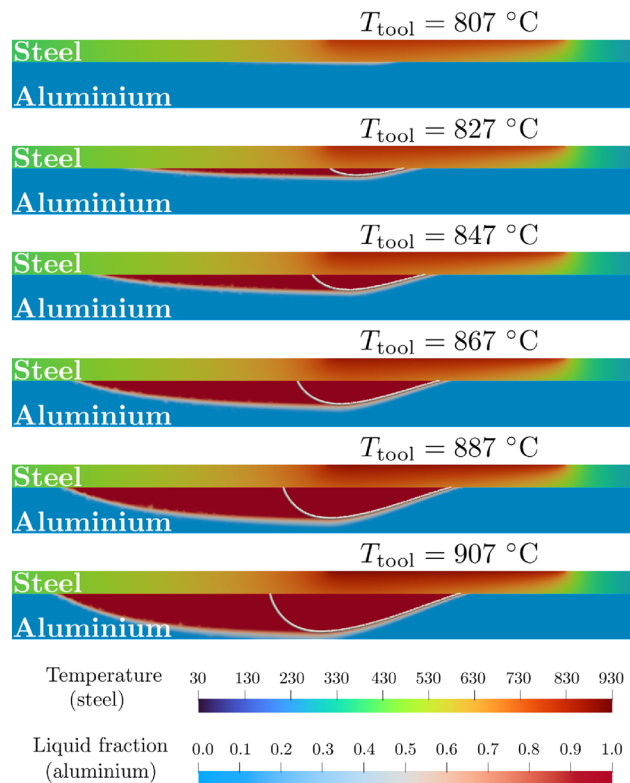
Fig. 11 Simulations for different tool temperatures but same travel speed of 200 mm/min. From each simulation, the melt pool geometry is measured to create the graph in Fig. 12
