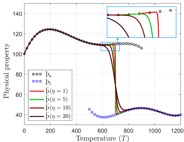
Fig. 20 Smoothing of a physical parameter in the phase change zone. Dots represent polynomial functions that fit and extrapolate some experimental points. The solid lines are the smooth continuous functions ( \tilde{\mathfrak{p}} ) that define the physical parameter over the entire temperature range
