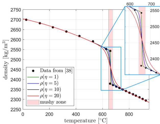
Fig. 8 Temperature-dependent density curves. \eta represents a parameter defining the smoothness of a Heaviside function defined in Appendix A
