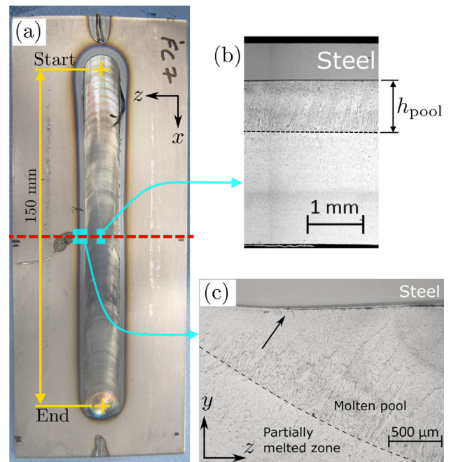
Fig. 7 FMB experimental sample. a The steel plate is observed from the top. The heat affected zone and the damage caused by friction are visible on the steel plate. b Typical views by light microscopy. Subfigures (b) and (c) are retrieved from [4]
