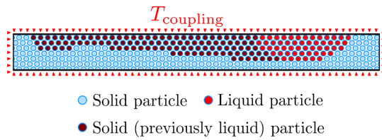
Fig. 5 Thermal boundary condition of the PFEM sub-model and illustration of the space discretisation using particles
