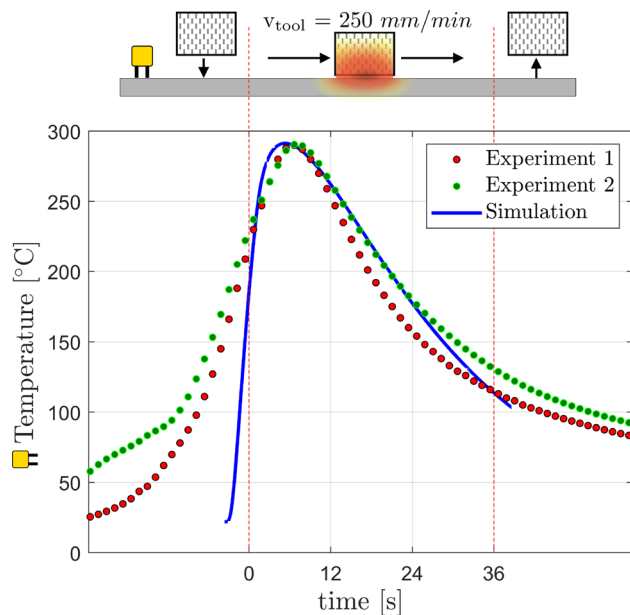
Fig. 16 Temperature of a thermocouple placed between the left edge of the plate and the initial position of the tool, as shown in the sketch over the graph. The simulation uses a preheating time of 4.0 s
