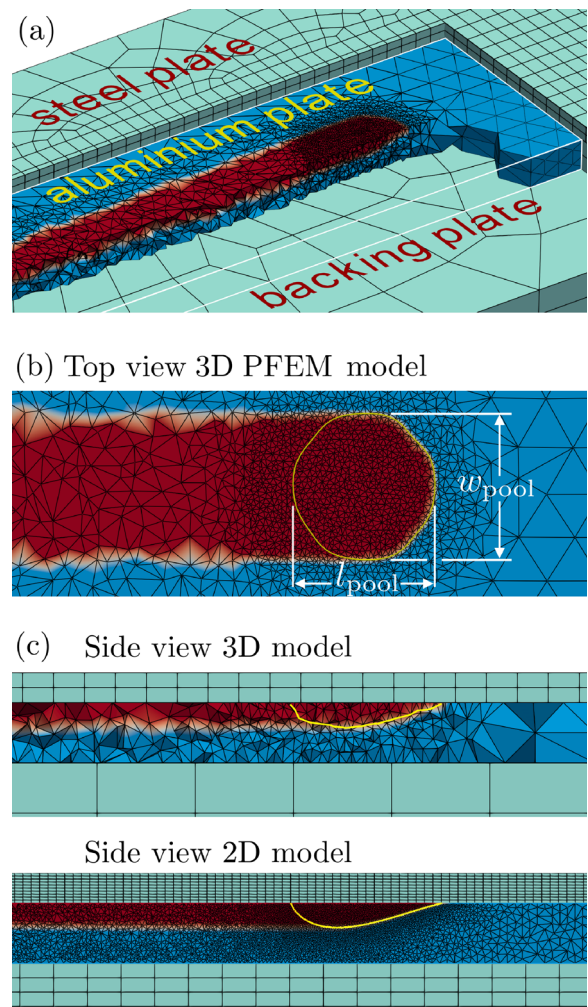
Fig. 10 a Perspective view of the 3D model, with sectioning of the steel and aluminium plates to illustrate the spatial discretisation. b Top view denoting the width and length of the melt pool. c Side view of the symmetry plane of the 3D model, placed above the 2D model for comparison. The aluminium plate shows the liquid fraction history
