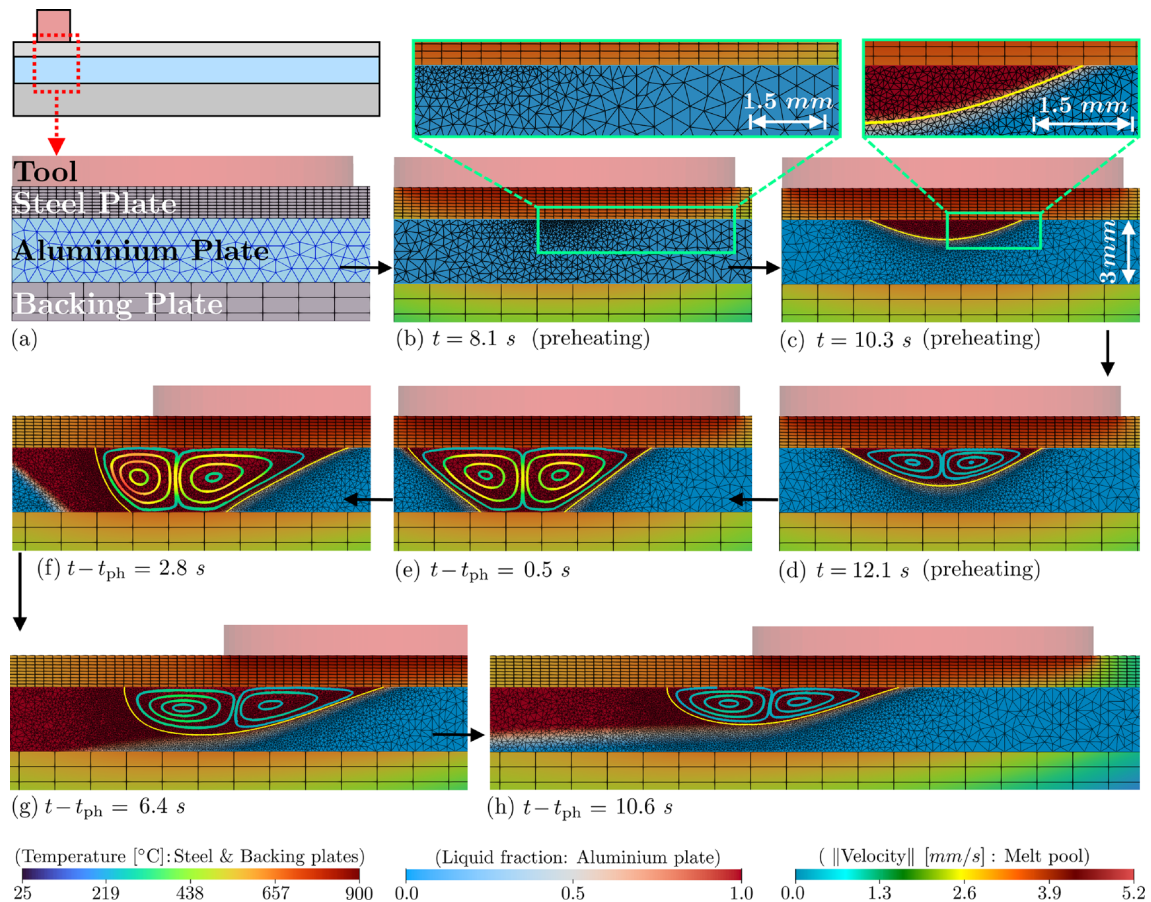
Fig. 9 Simulation of the FMB process using a partitioned FEM + PFEM approach. a The initial discretisation. b Temperature in the aluminium plate approaches the melting point and element size is adapted in the PFEM zone. c Melt pool appears. d Melt pool starts flowing due to natural convection. e The preheating phase is completed and the tool begins to move horizontally while the melt pool reaches the full thickness of
