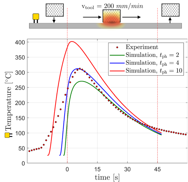
Fig. 15 Temperature of a thermocouple placed between the left edge of the plate and the initial position of the tool, as shown in the sketch over the graph. Three simulations are plotted with different preheating times t_{ph} (given in seconds). t_{ph} = 4 \text{ s} leads to the same maximum temperature recorded experimentally
