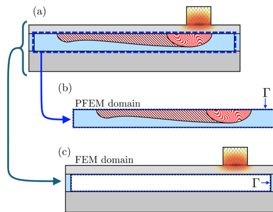
Fig. 2 Illustration of the FMB domain partition used in this work. a The complete FMB domain, b the PFEM domain and c the FEM domain. \Gamma denotes the common surface between FEM and PFEM domains
