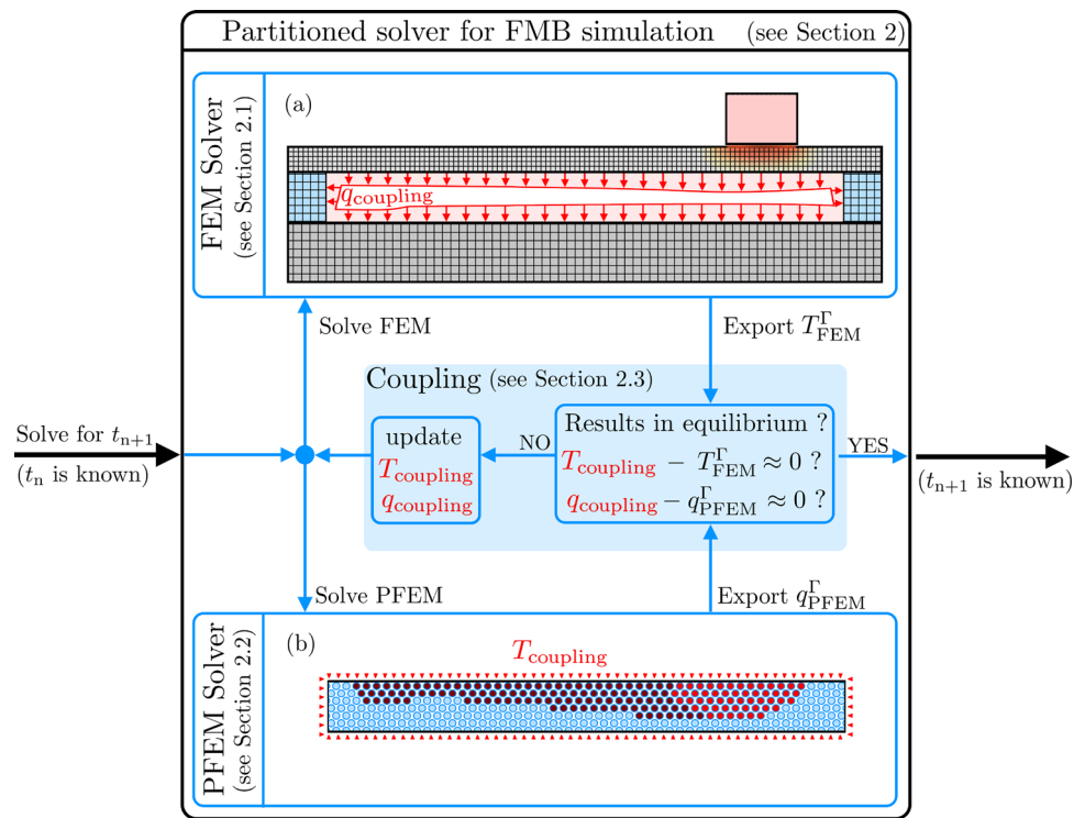
Fig. 6 Illustration of the proposed numerical approach to simulate the FMB process. a Domain solved by the Finite Element Method (FEM). b Domain solved by the Particle Finite Element Method (PFEM). The light blue box represents the coupling between the FEM and PFEM solvers in a Dirichlet-Neumann approach. \Gamma denotes the interface between the FEM and PFEM models (see Fig. 2). Only the thermal part of the coupling is illustrated here
