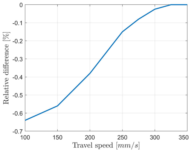
Fig. 18 Relative difference in melt pool depth between flowing and non-flowing melt pool models
